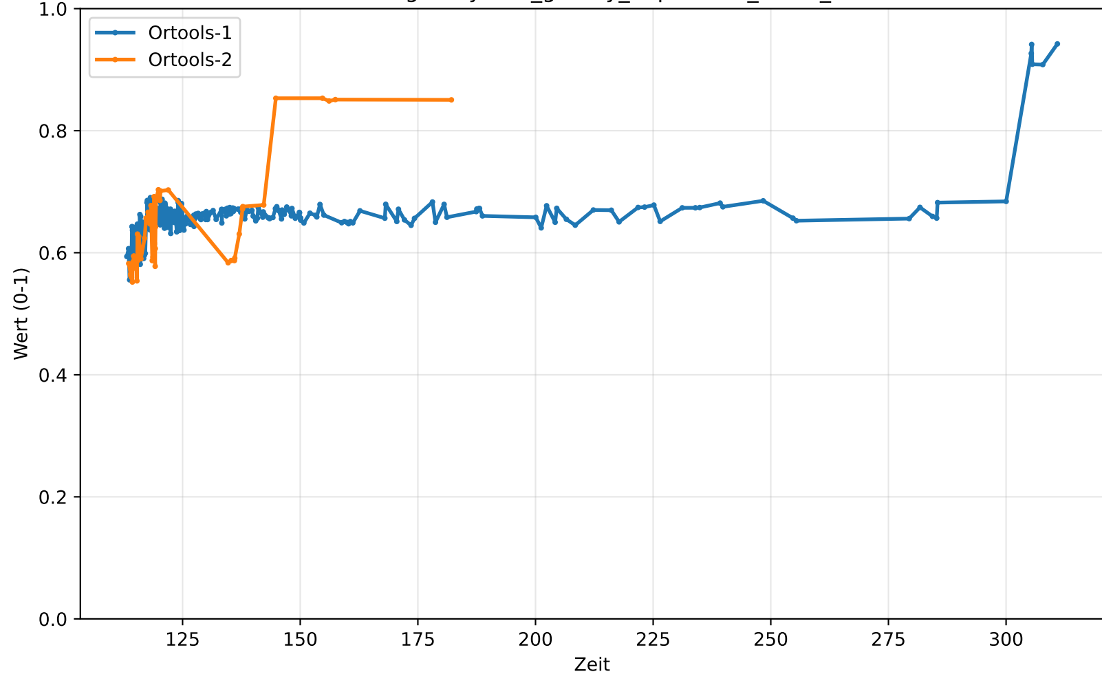
Instanz: greedy/038_greedy_impossible_move_120
