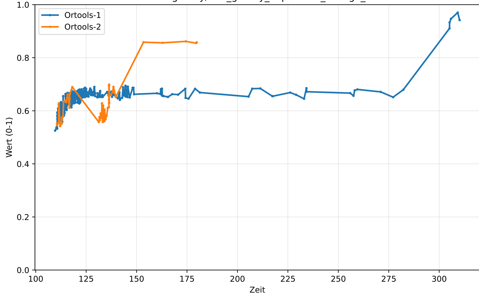
Instanz: greedy/039_greedy_impossible_change_120
