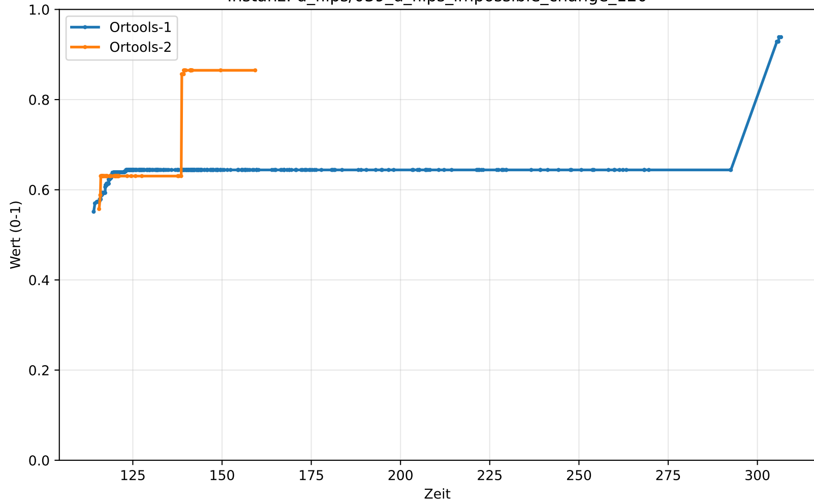
Instanz: d_flips/039_d_flips_impossible_change_120
