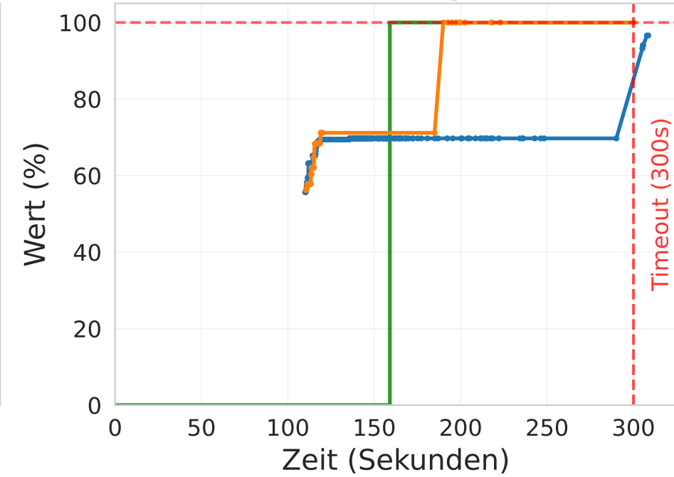
Greedy
