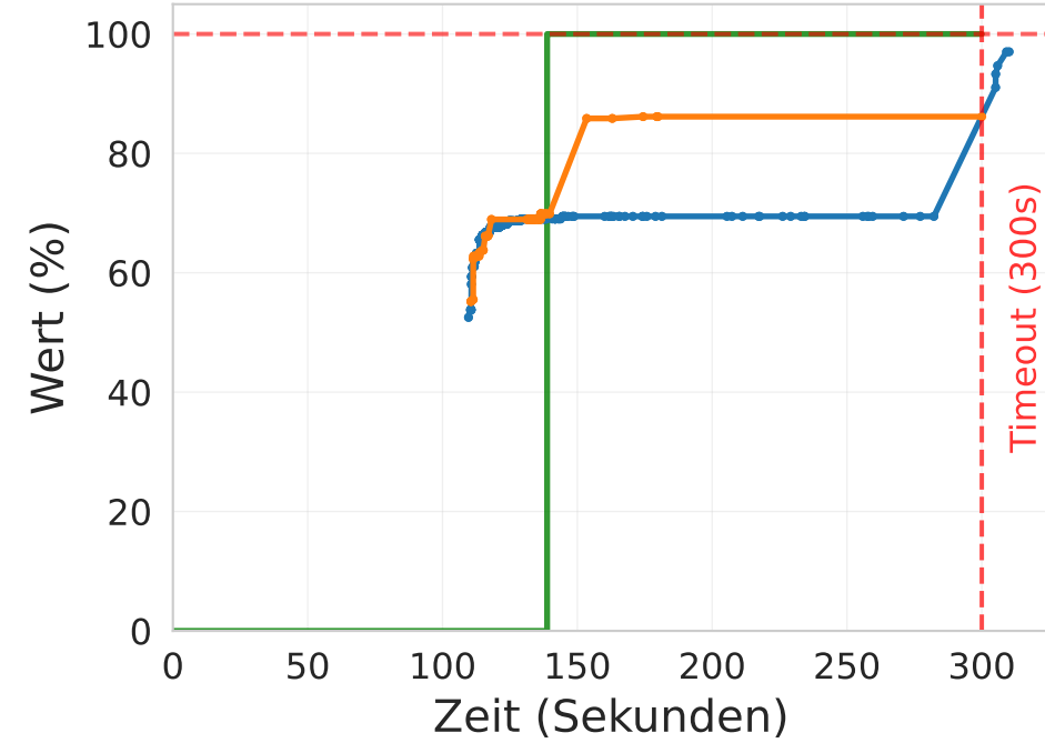
Greedy
