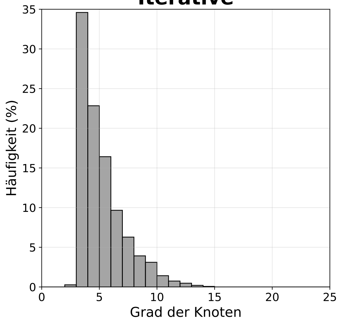
Iterative
