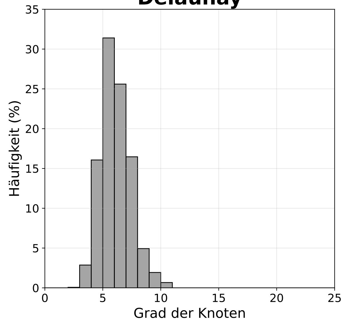
Delaunay
