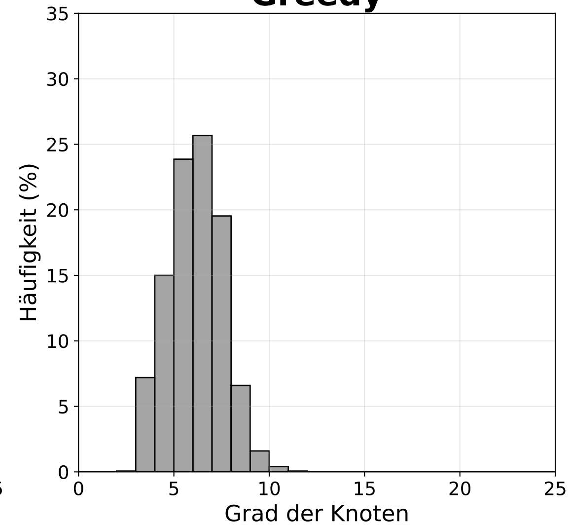
Greedy
