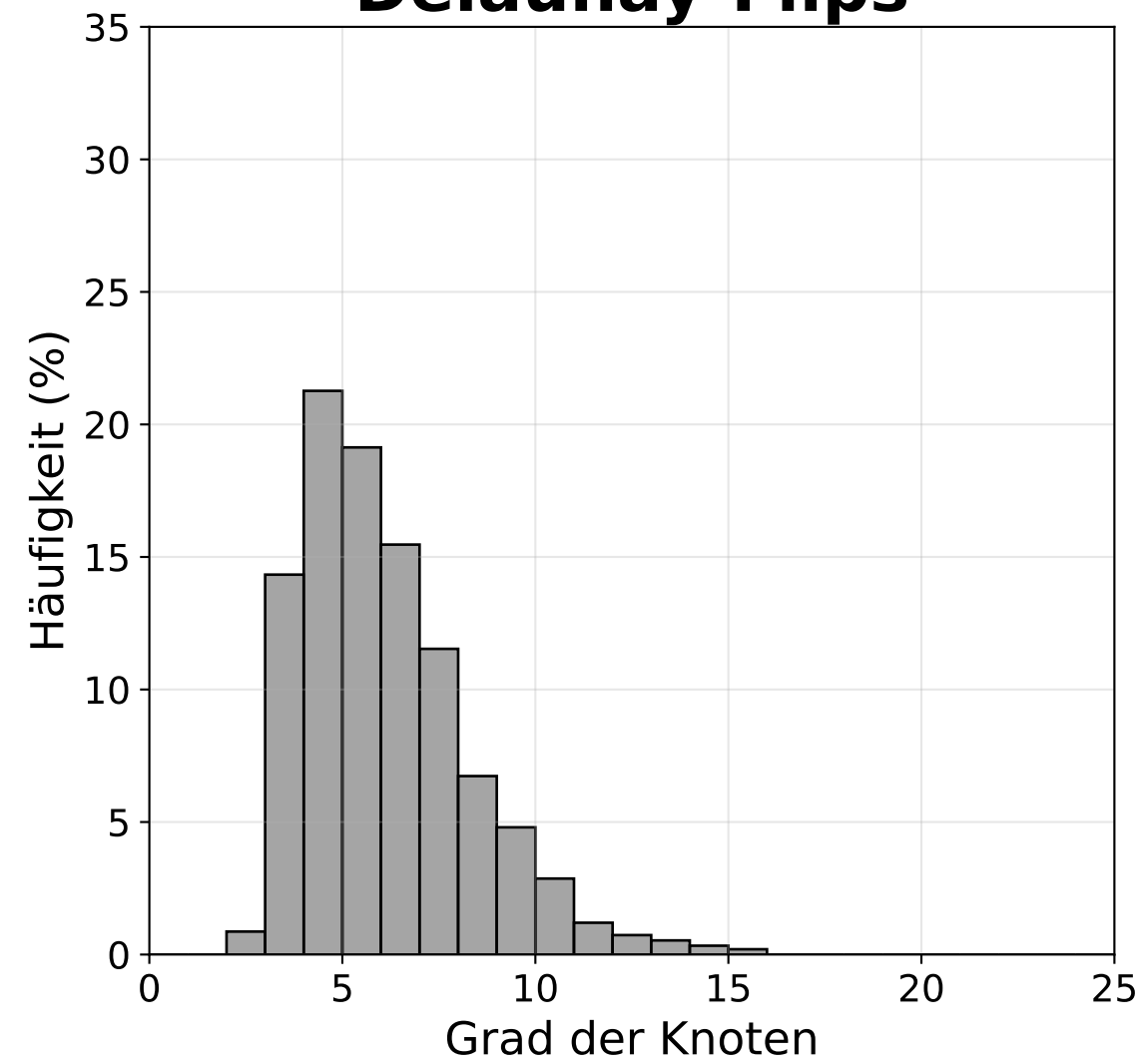
Delaunay
