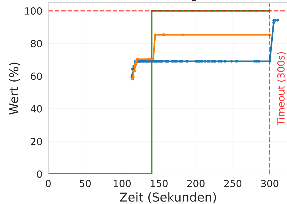
Greedy
