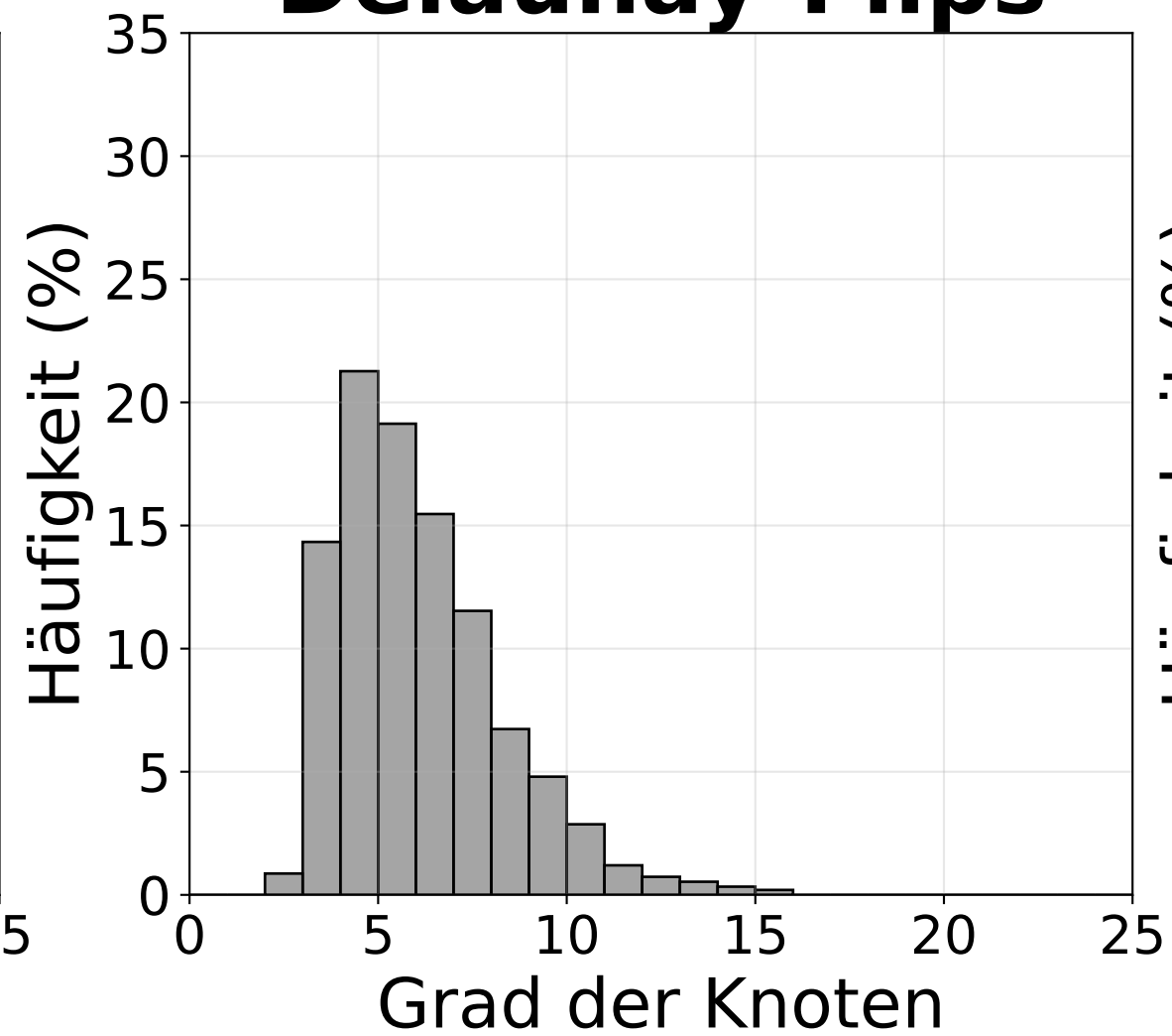
Delaunay
