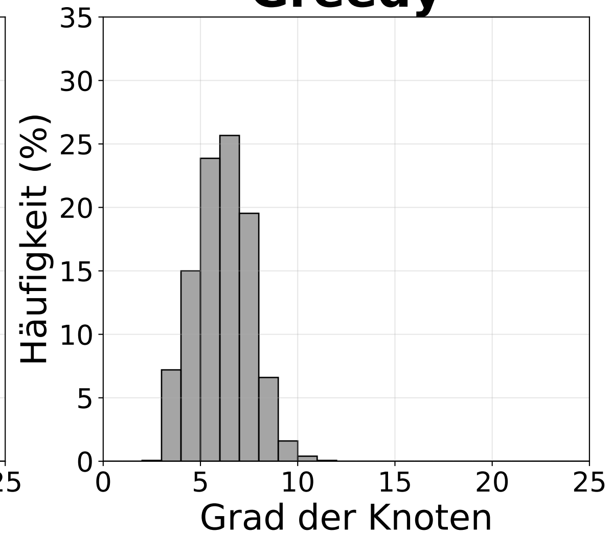
Greedy
