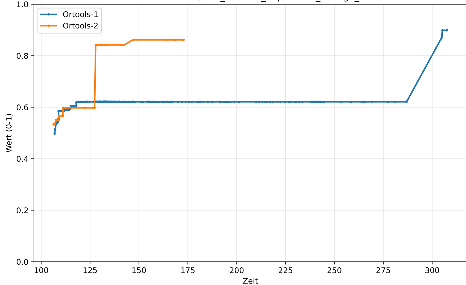
Instanz: random/039_random_impossible_change_120
