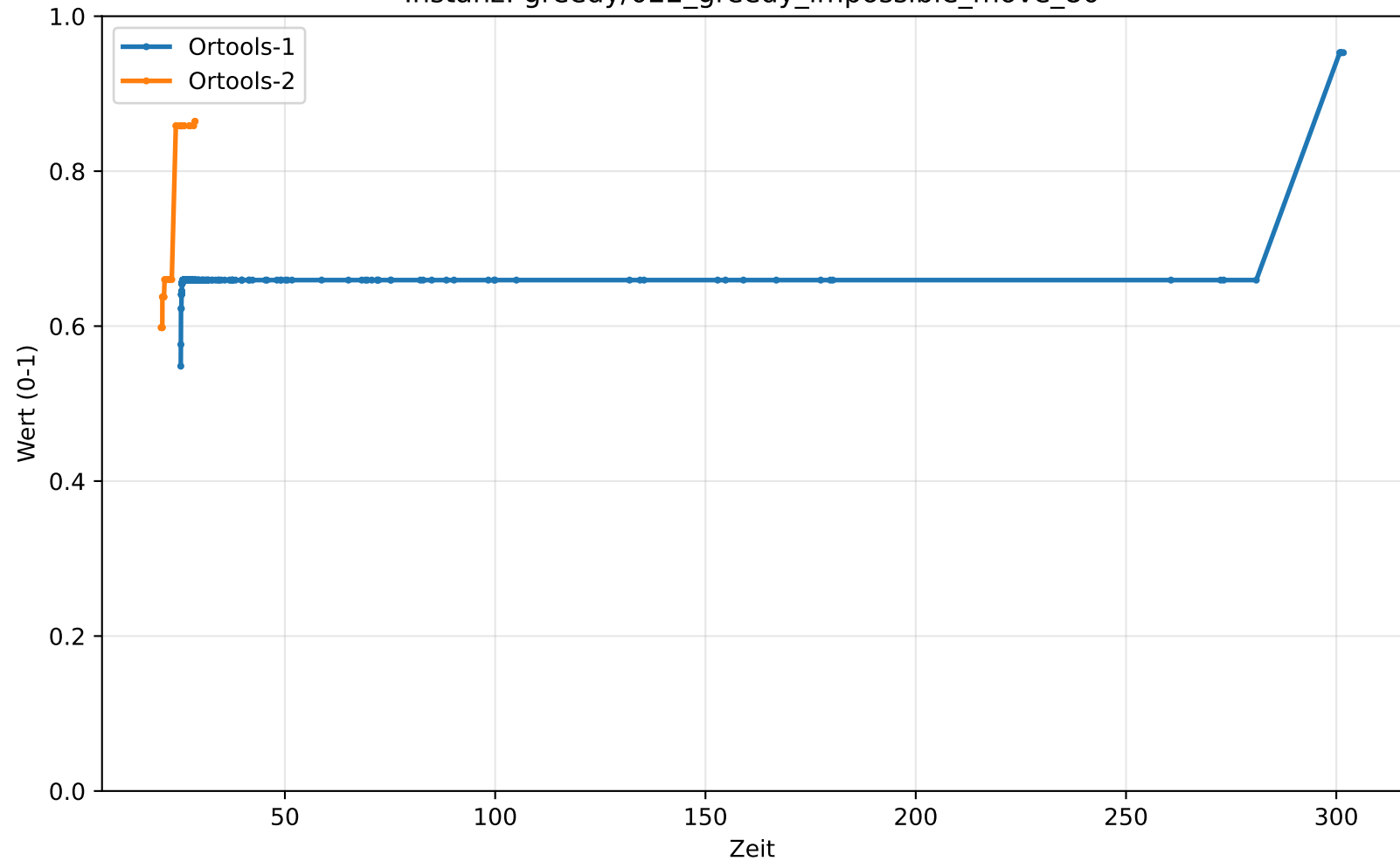
Instanz: greedy/022_greedy_impossible_move_80
