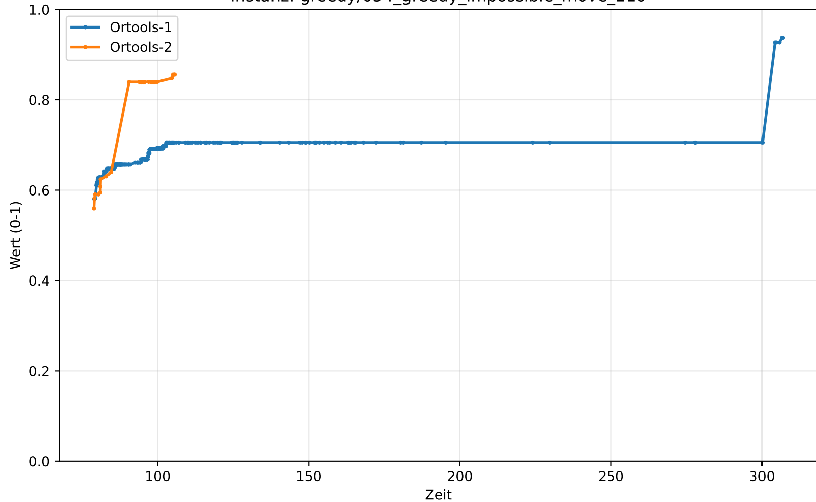
Instanz: greedy/034_greedy_impossible_move_110
