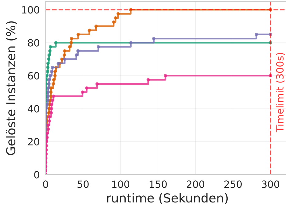
Delaunay-Flips
