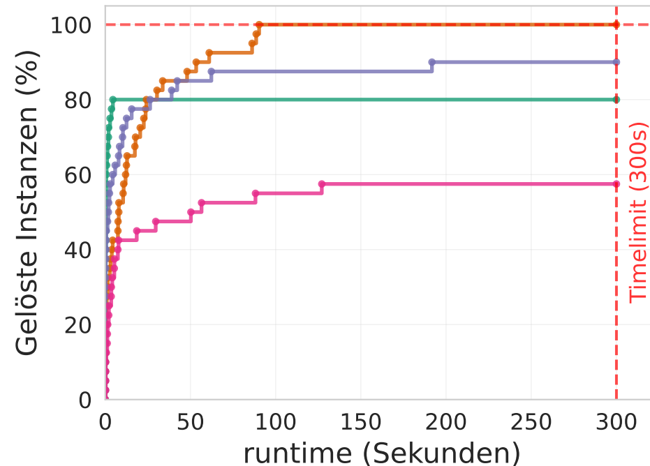
Random
