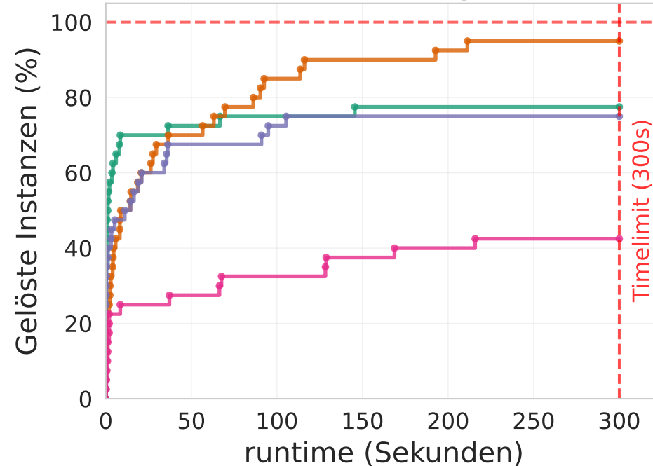
Delaunay
