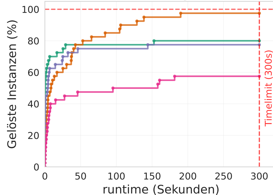
Greedy
