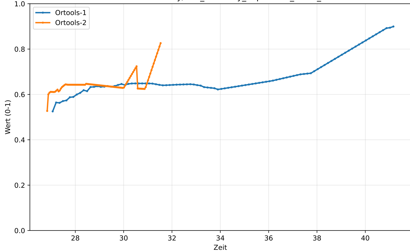
Instanz: delaunay/018_delaunay_impossible_move_70
