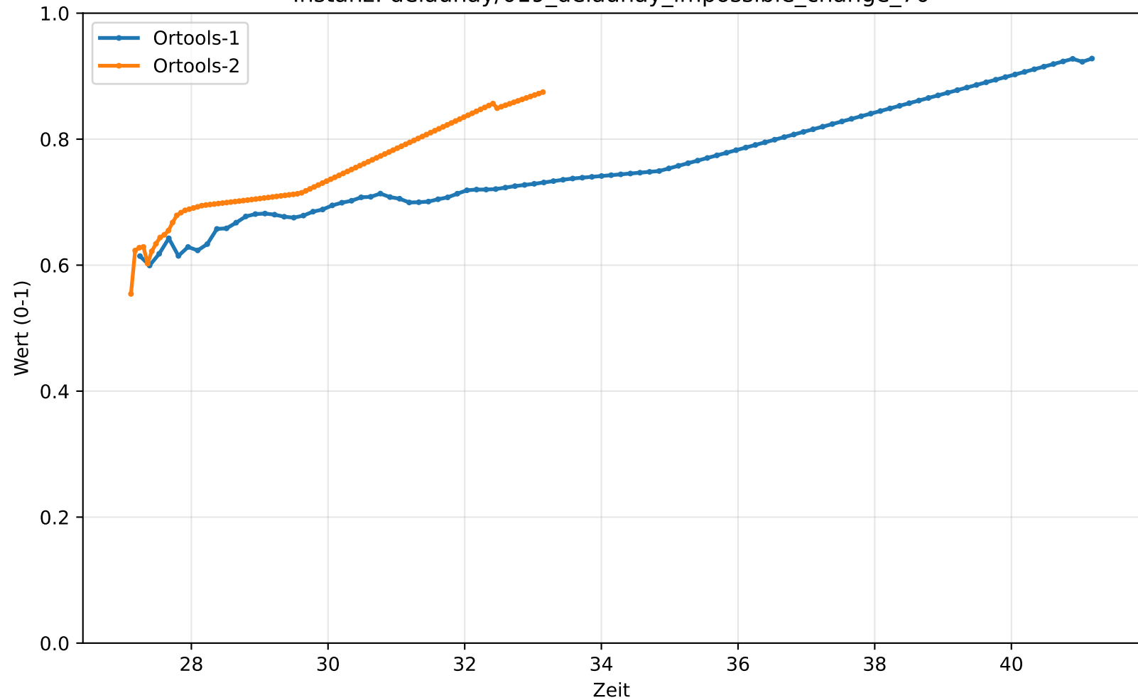
Instanz: delaunay/019_delaunay_impossible_change_70
