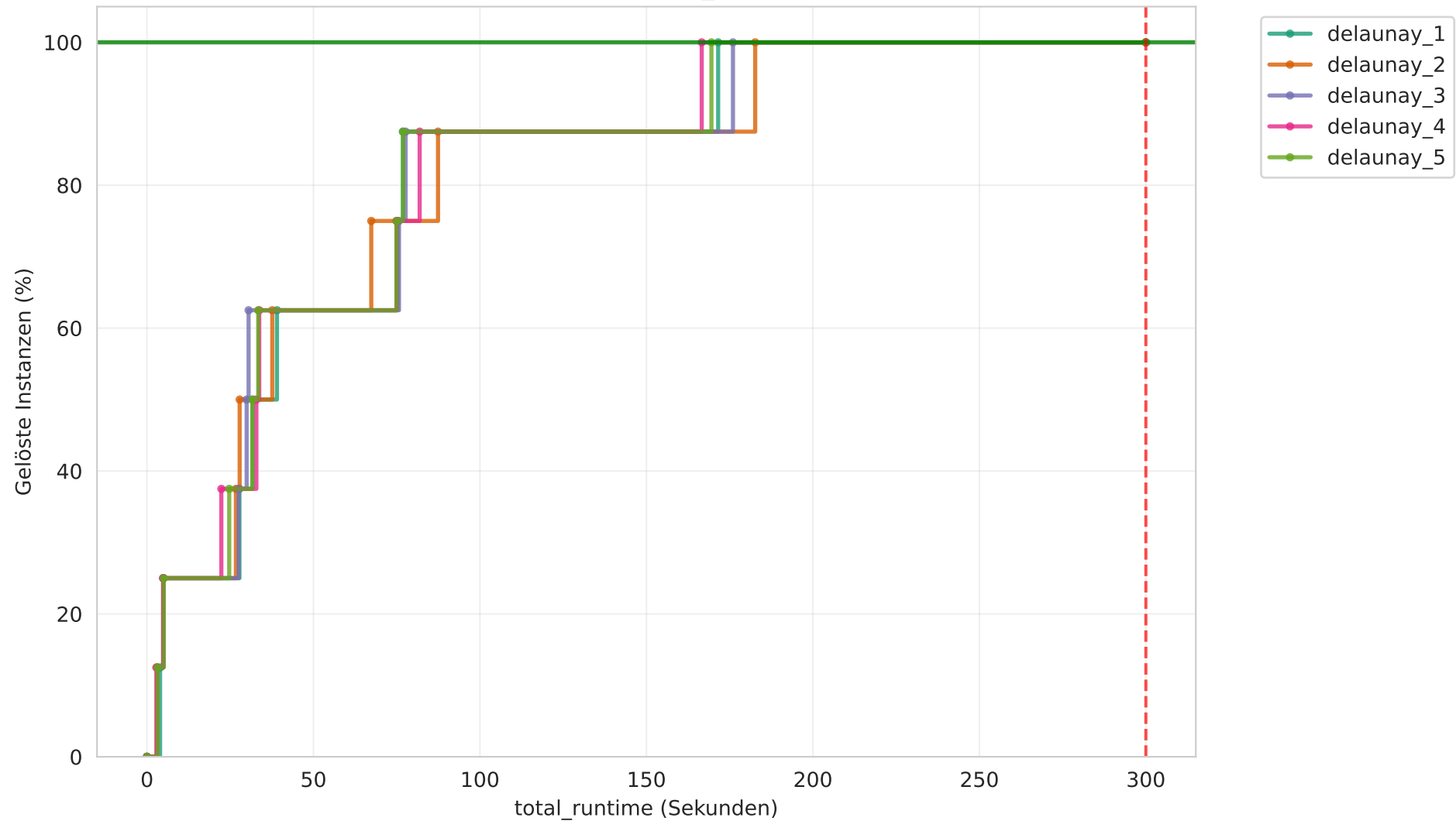
Cactus Plot - total_runtime
