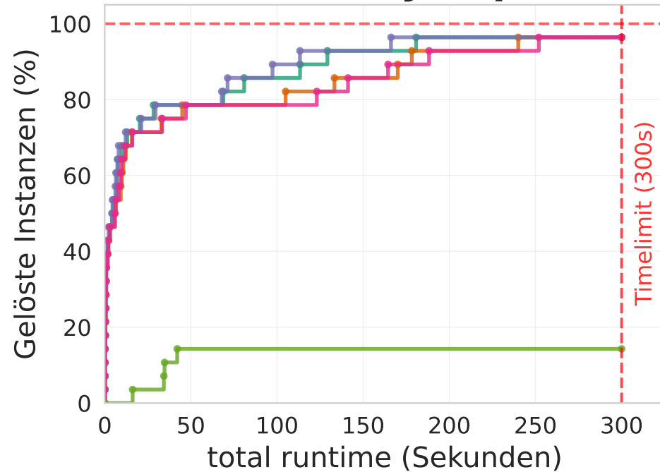
Iterative
