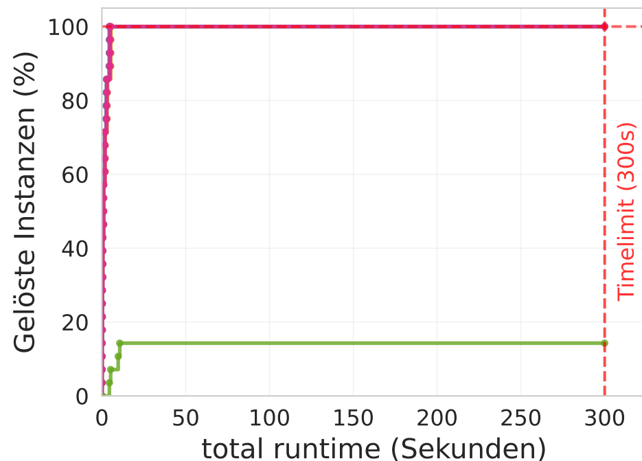
Iterative
