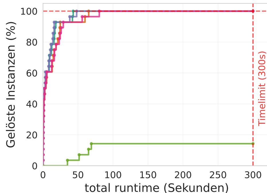
Random
