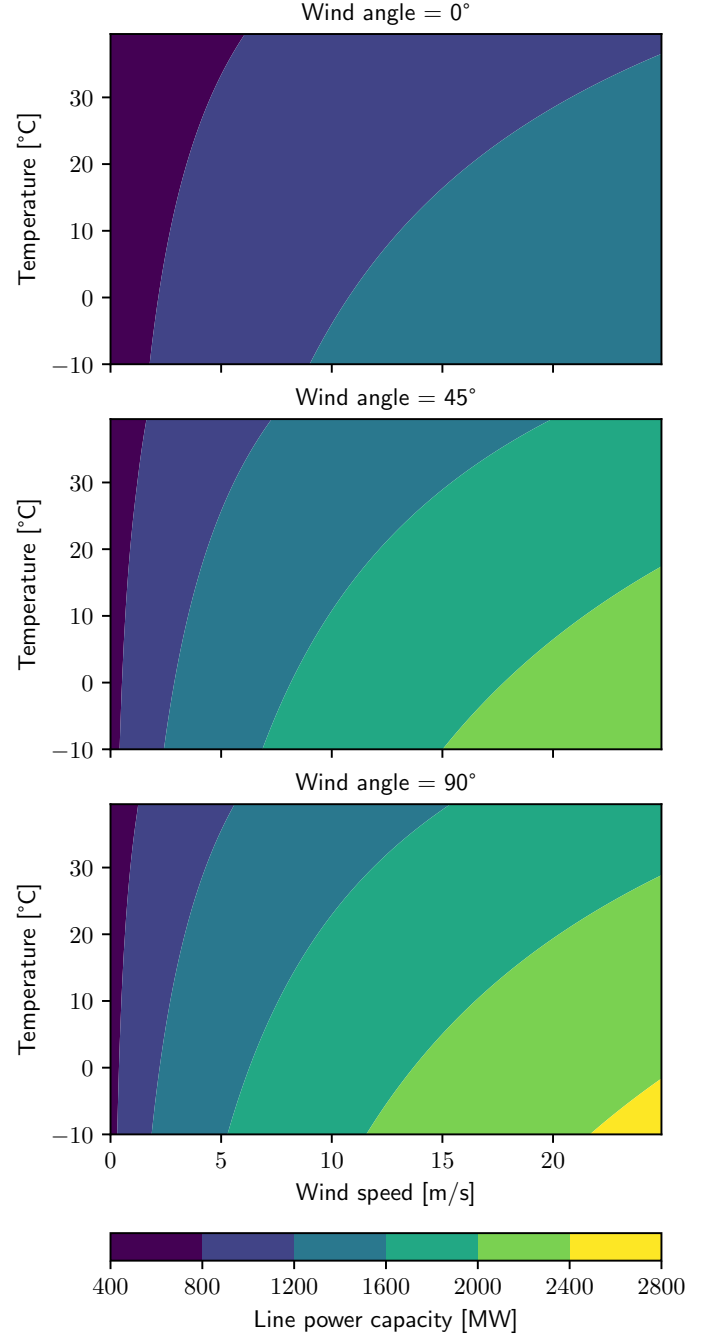
Figure 1: Power Rating for different prevailing weather conditions
