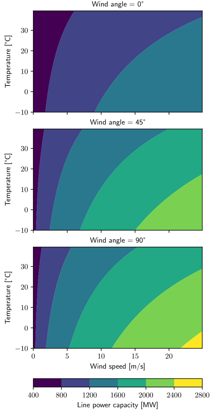
Figure 1: Power Rating for different prevailing weather conditions
