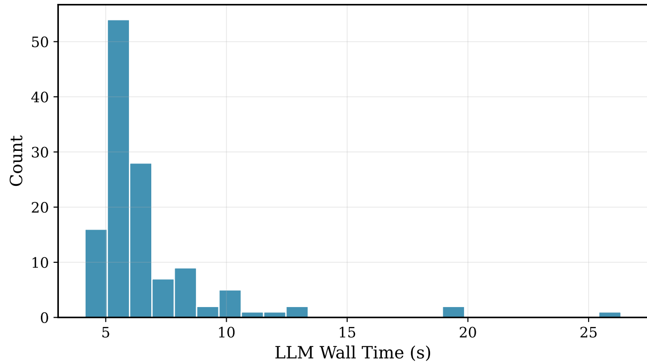
Pinned Run: LLM Wall-Time Distribution
