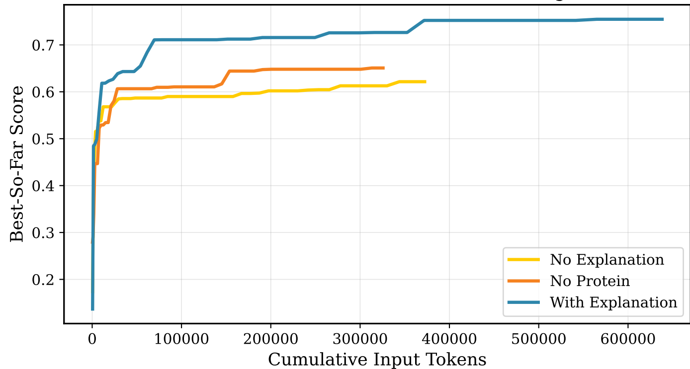
Boltz2 MGYB: Best-So-Far vs Cumulative Tokens (Higher is Better)
