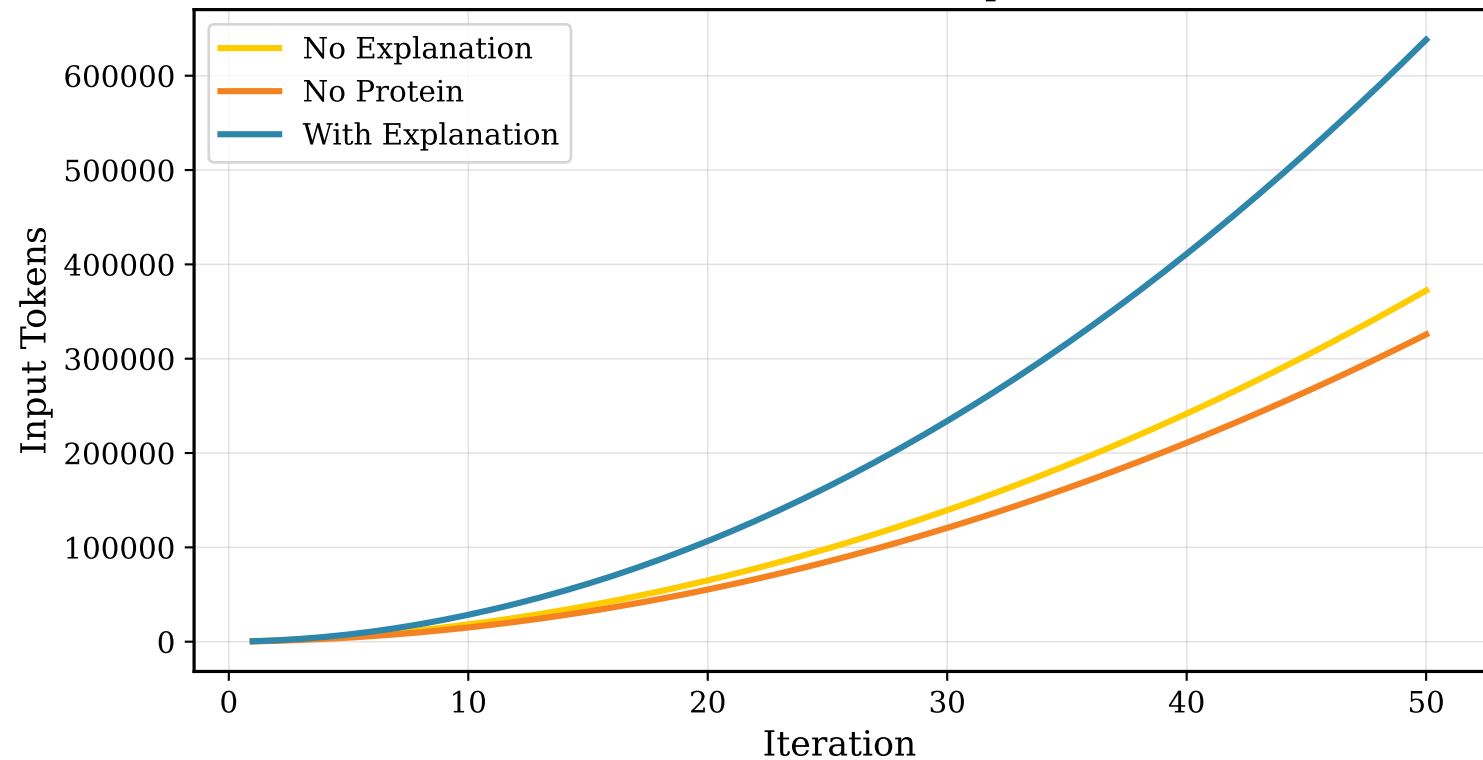
Boltz2: Cumulative Prompt Tokens
