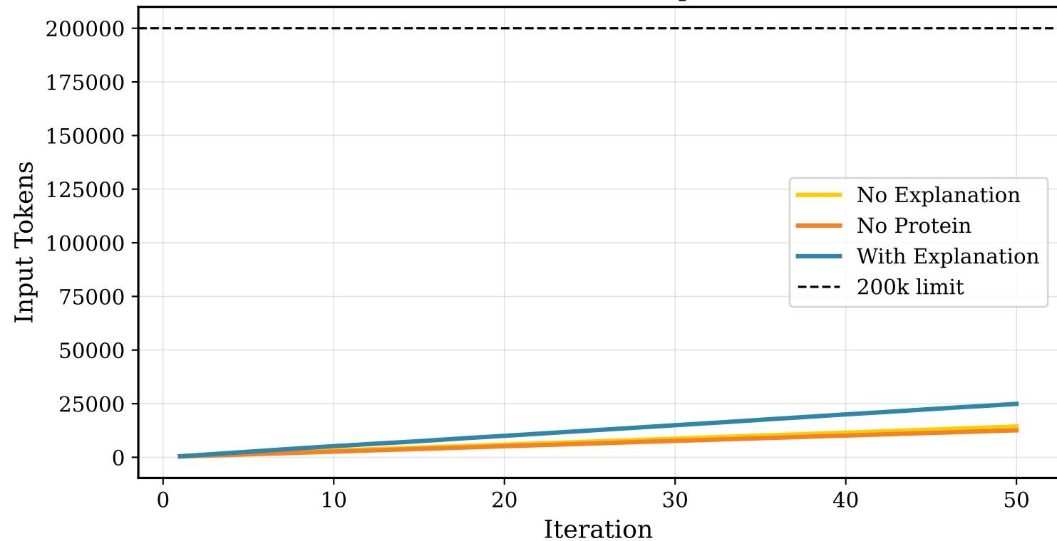
Boltz2: Current Prompt Tokens
