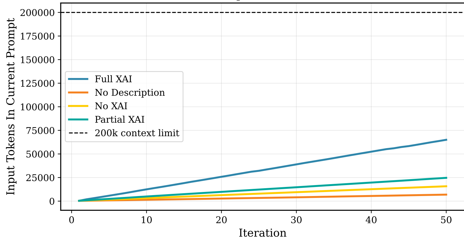
Current Prompt Size Over Iterations
