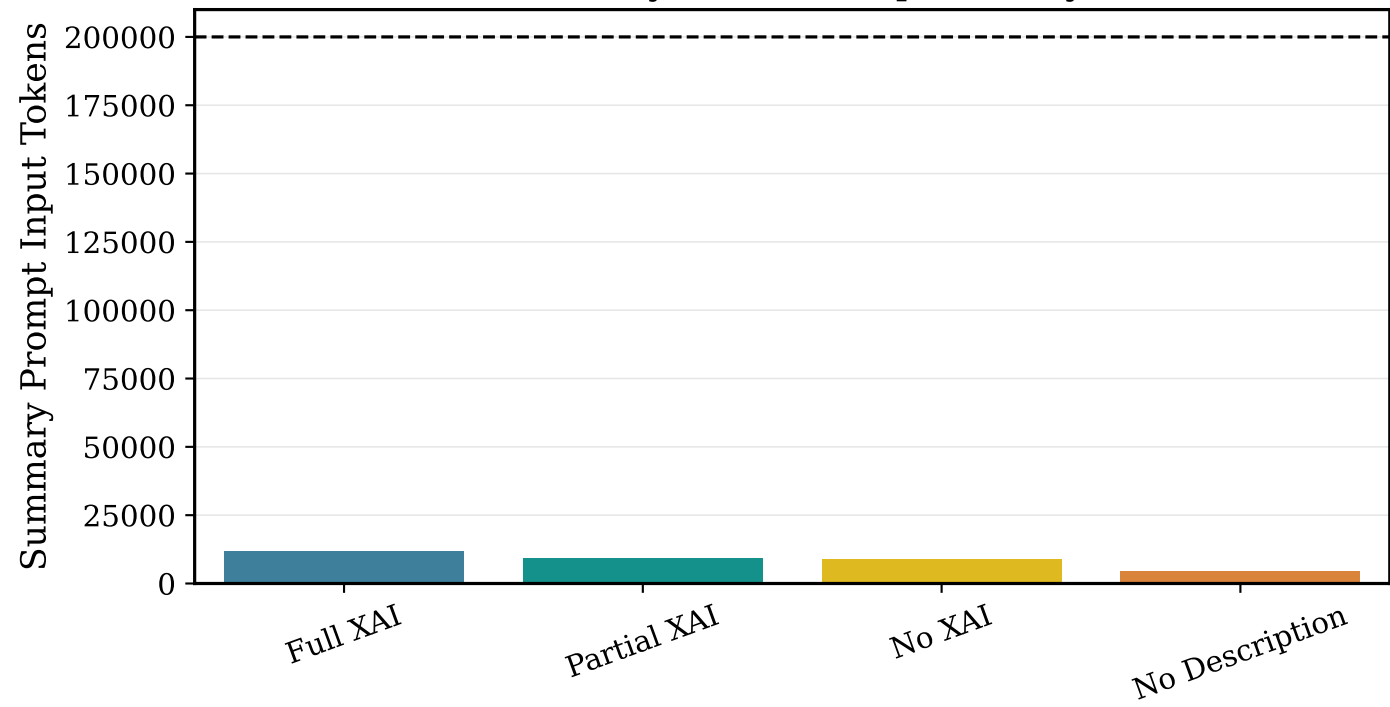
Final Summary-Node Prompt Size By Mode
