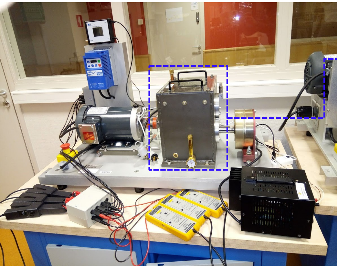
LASPI test bench
