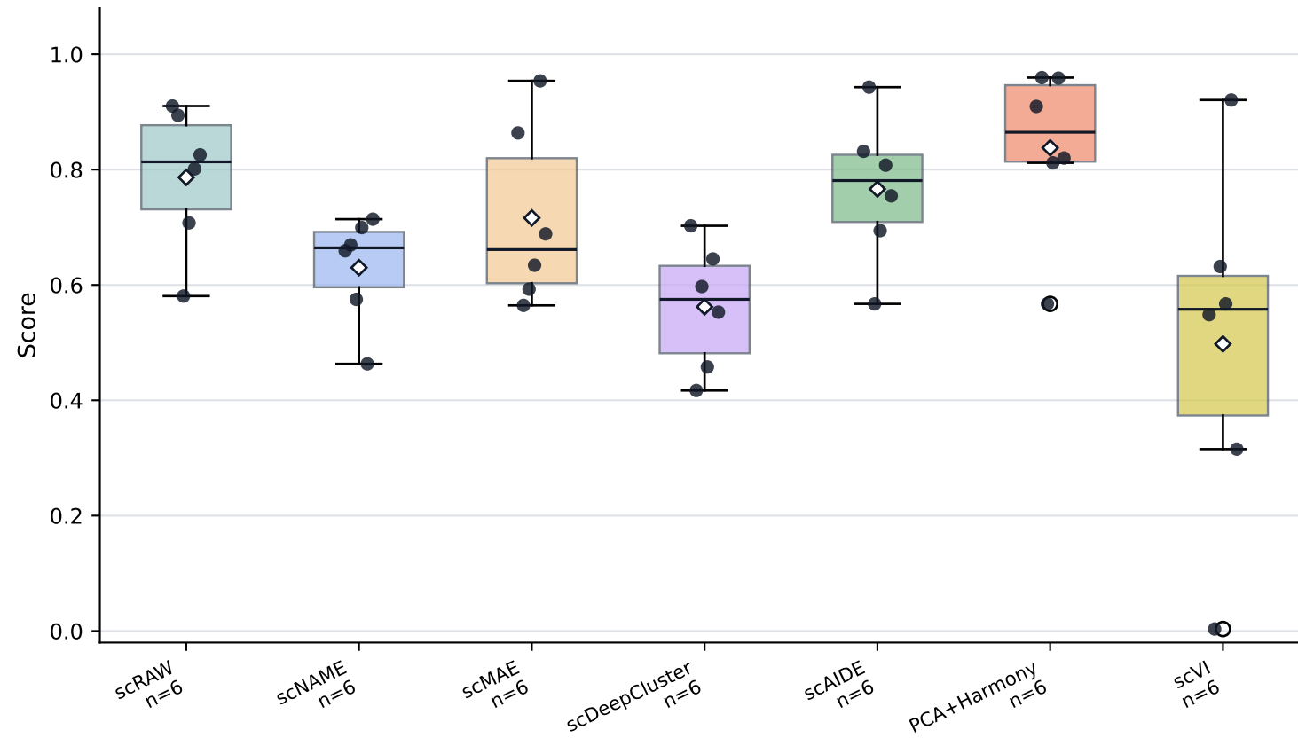
ARI
