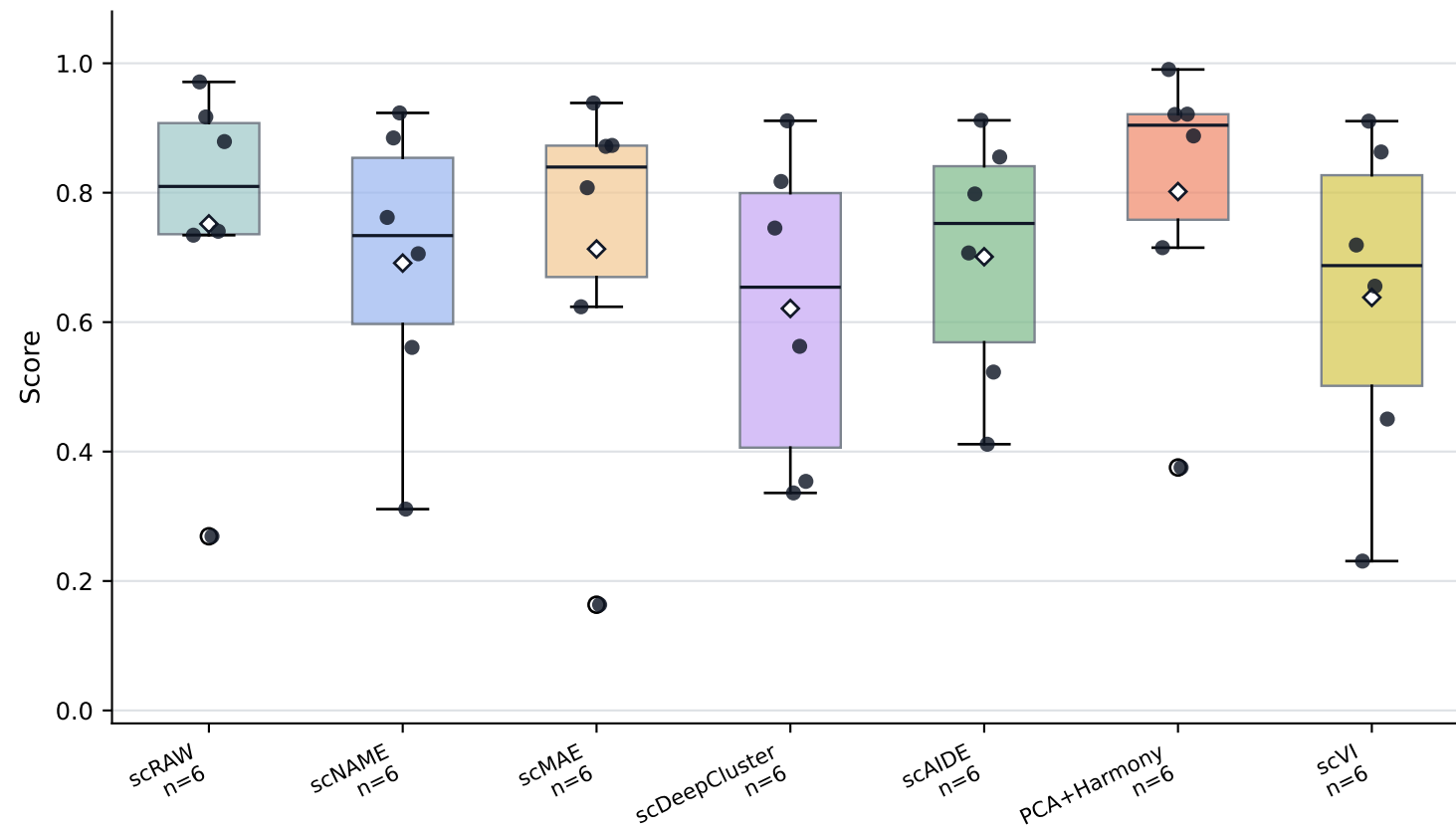
Rare ACC
