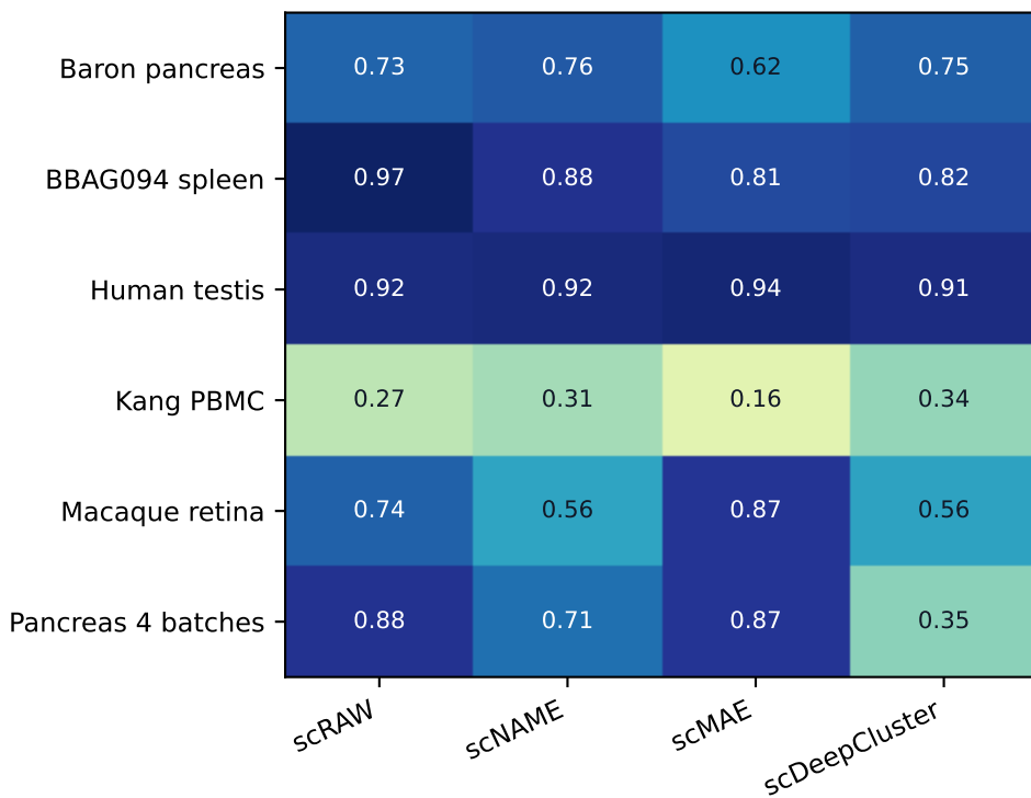
Rare ACC
