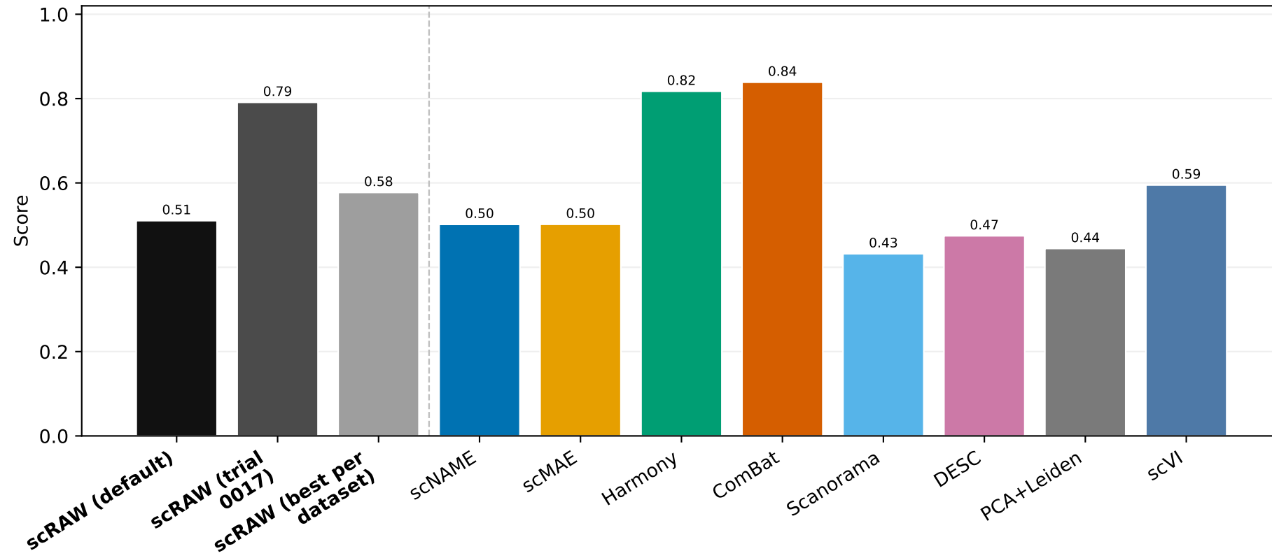
ARI
