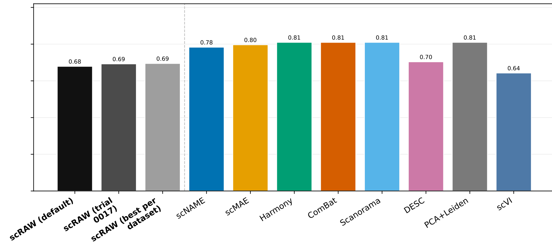
Balanced Acc
