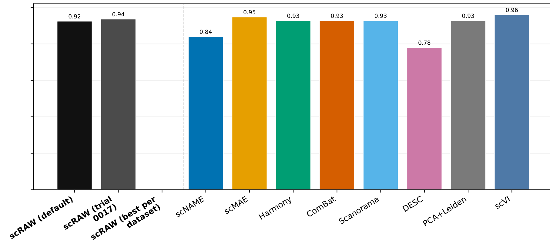
Batch correction
