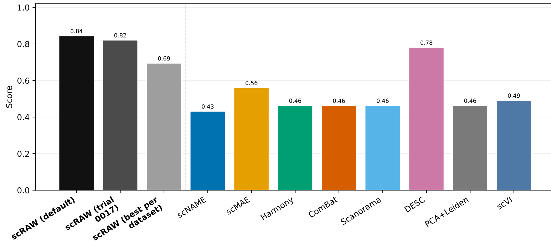
ARI
