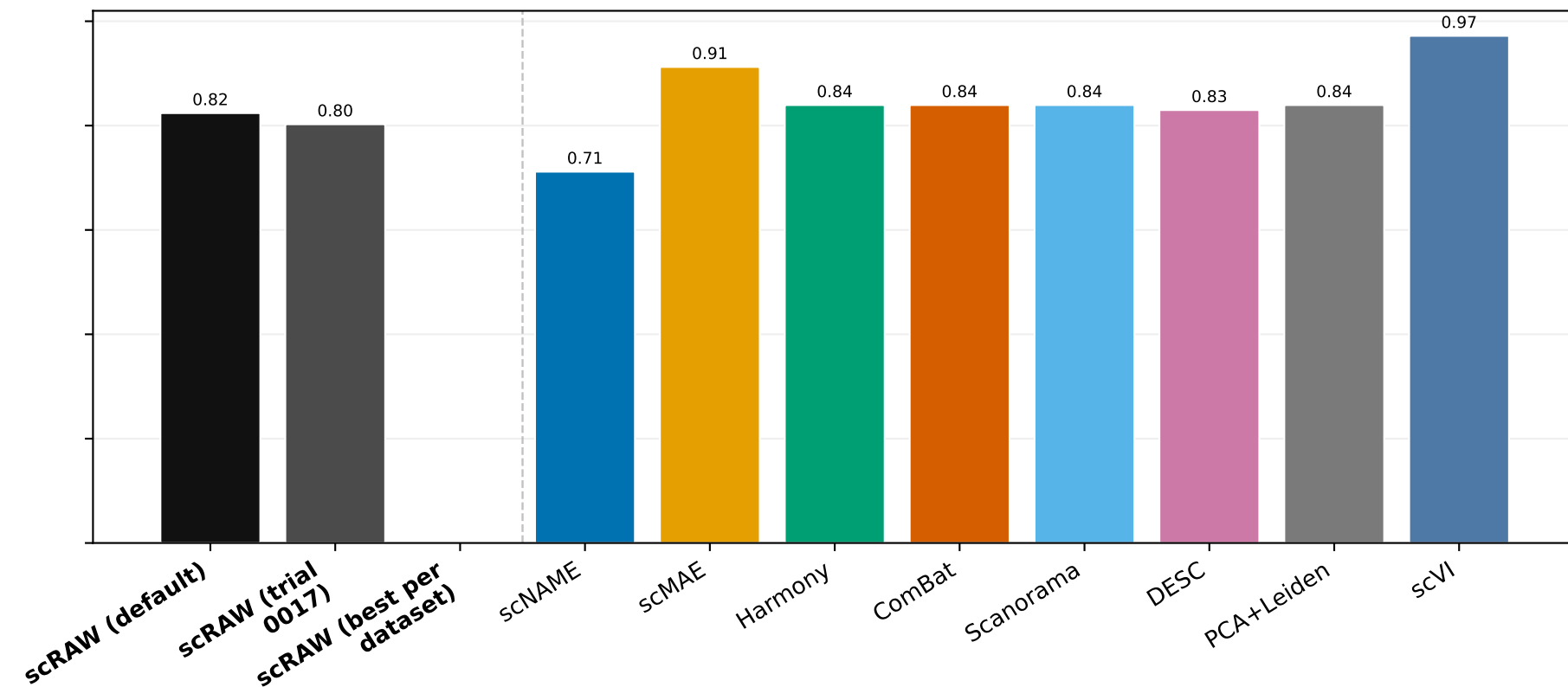
Batch correction
