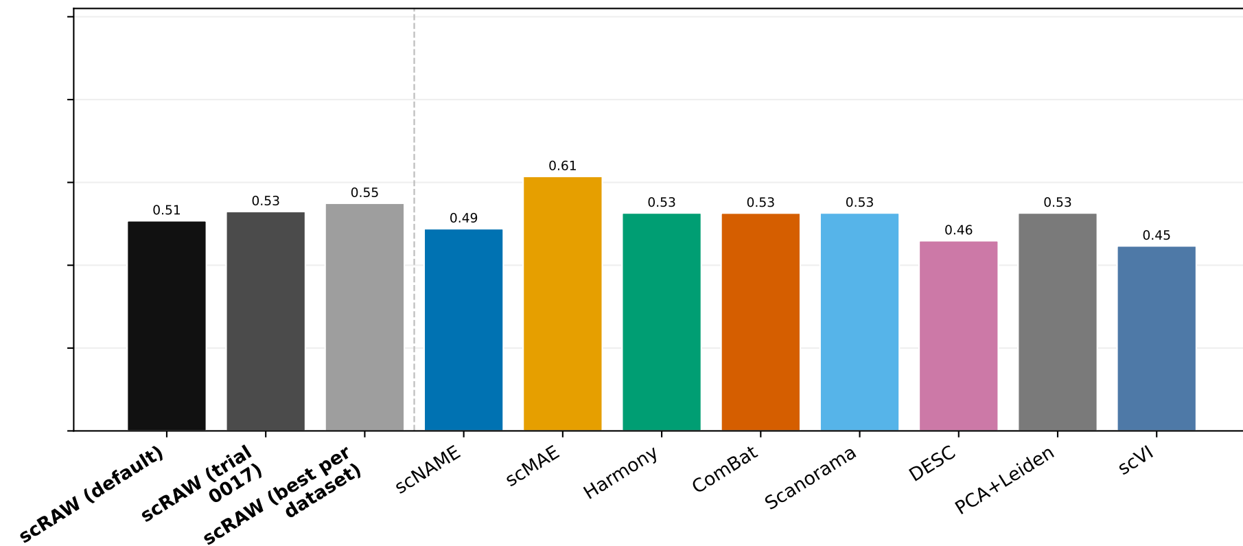
Balanced Acc
