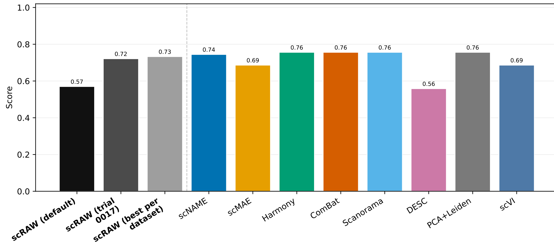
Rare Acc
