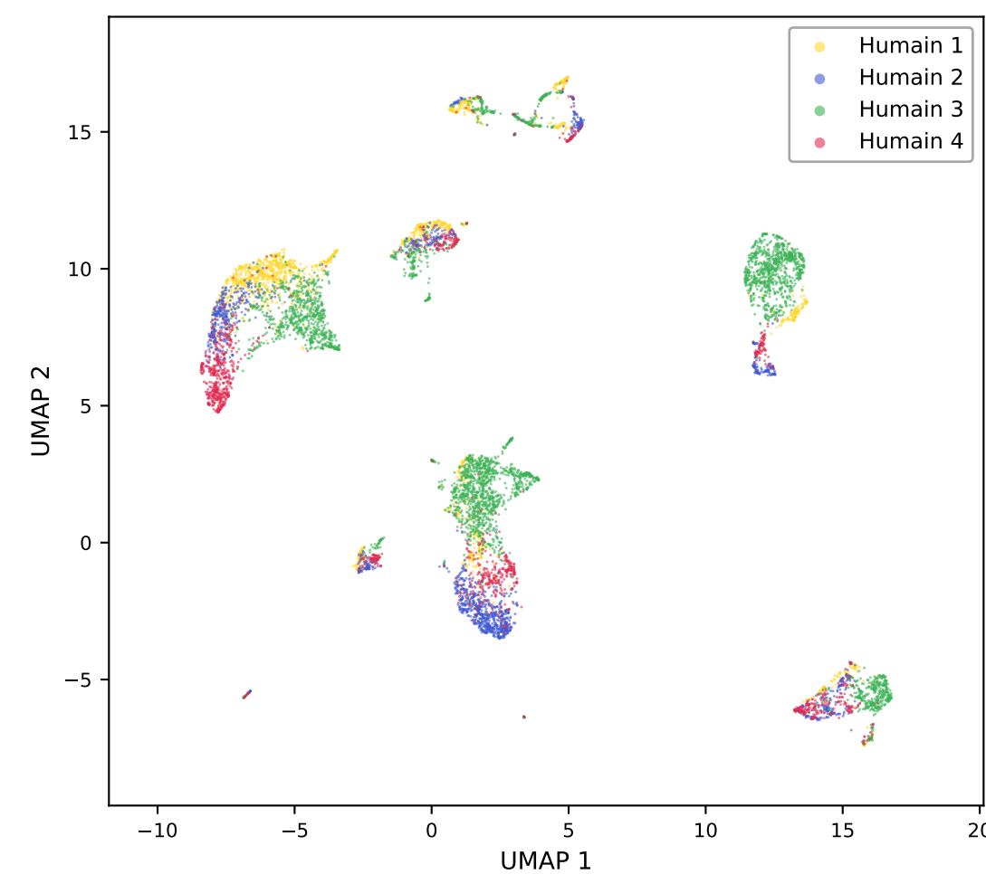
scMAE
