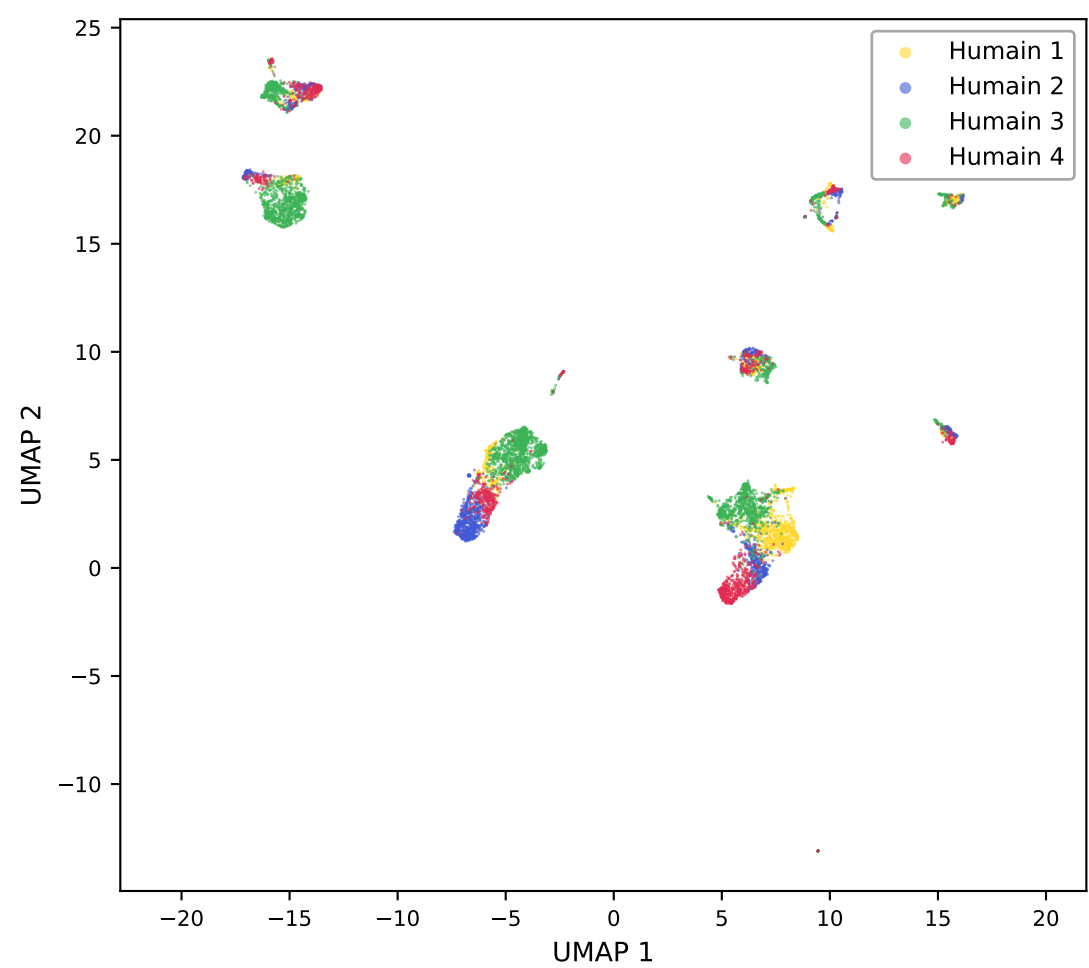
ComBat
