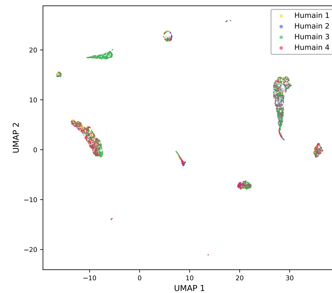
scRAW
