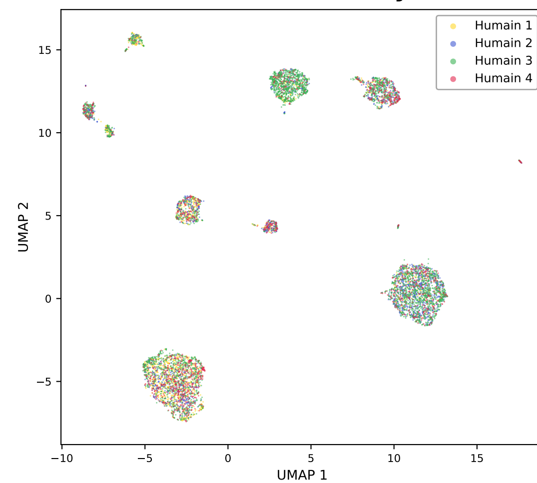
scVI + Harmony
