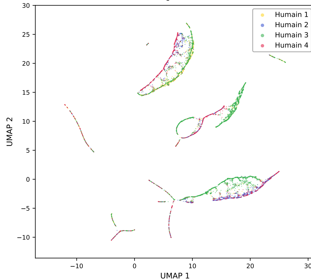
scDeepCluster
