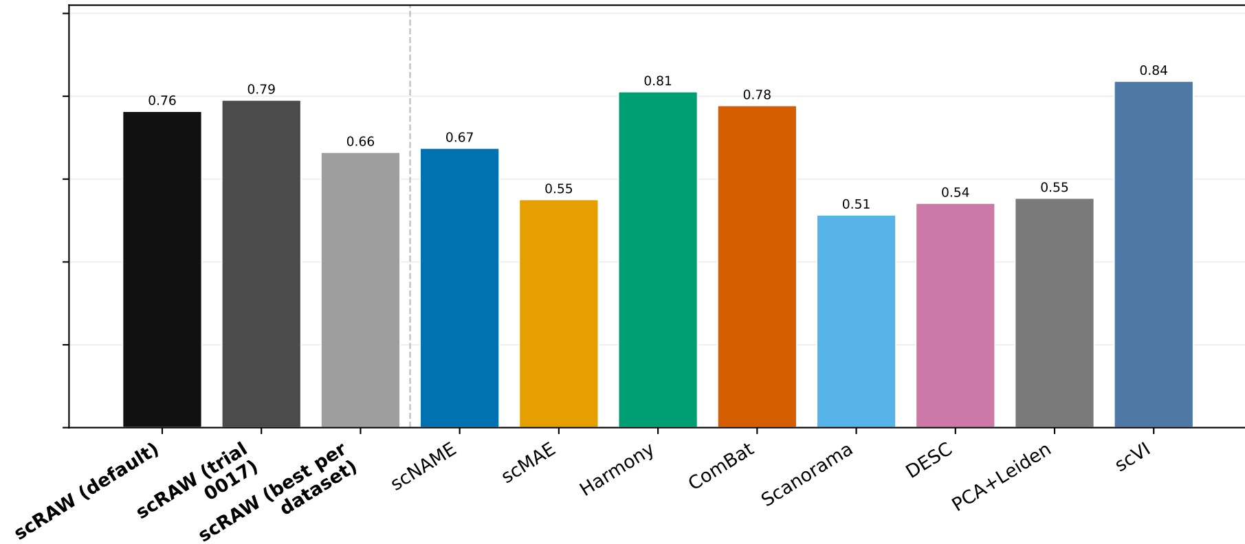
Batch correction
