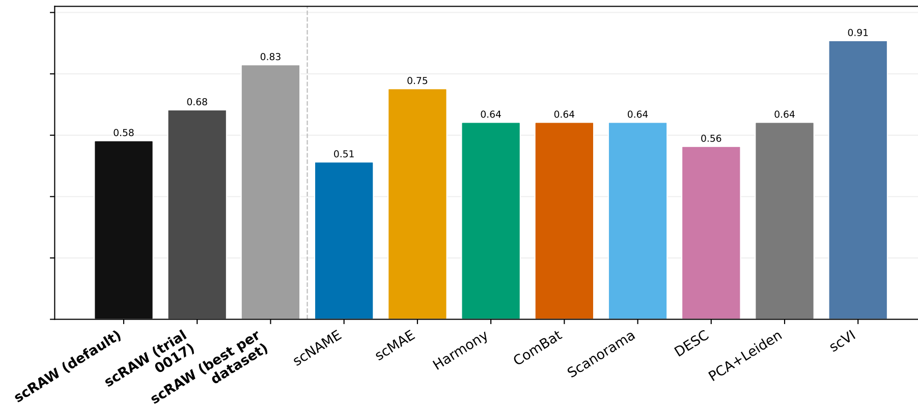
Batch correction
