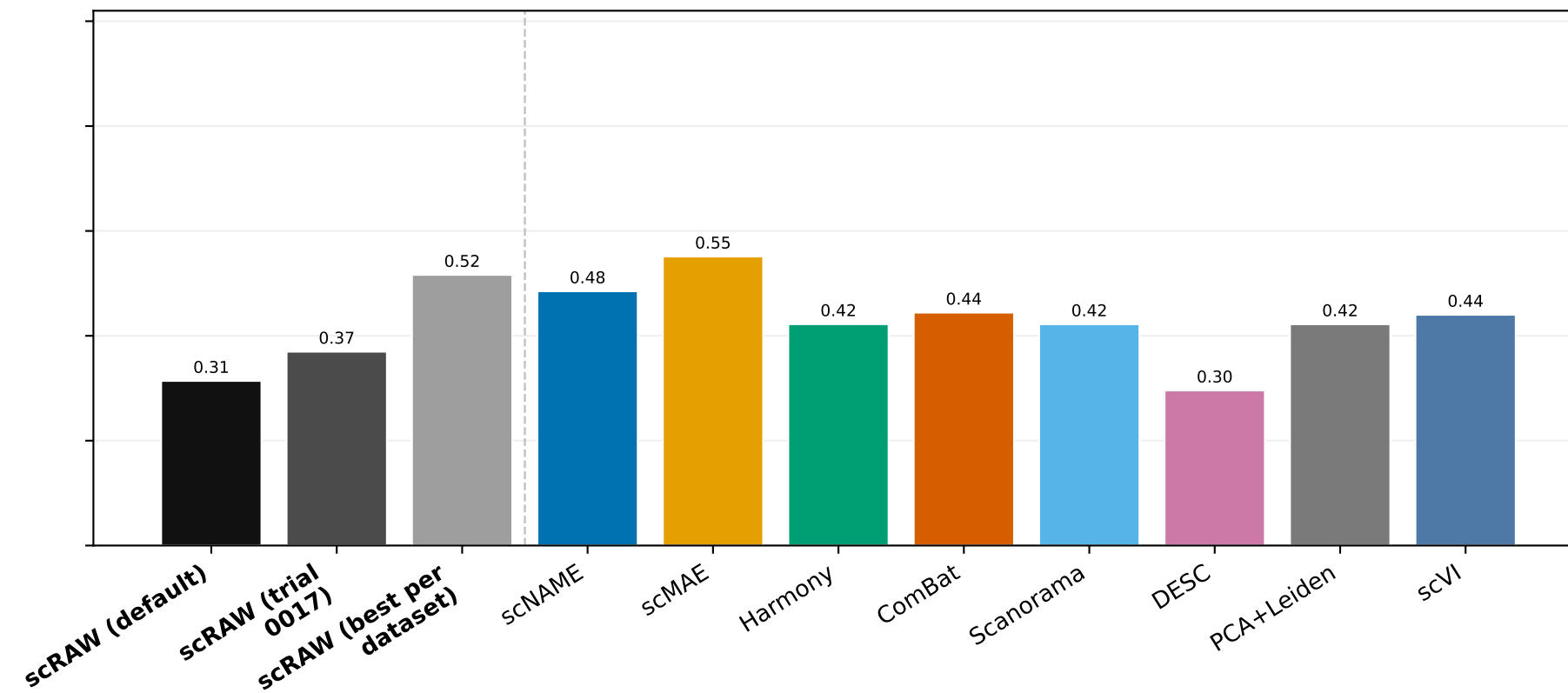
Balanced Acc
