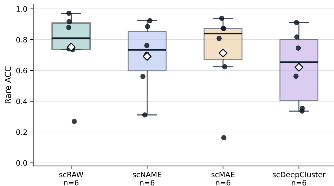
Rare ACC
