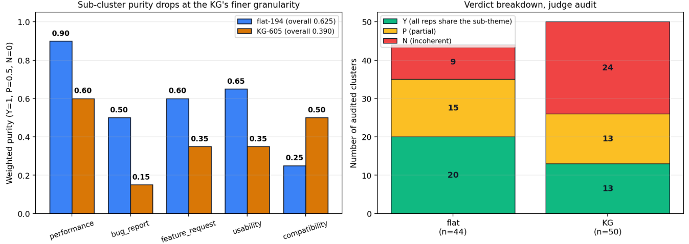
Figure 3: Extrinsic cluster purity for the flat baseline and the KG hierarchy, from the saved judge audit. Left: weighted purity per issue type, flat-194 against KG-605. The KG loses on four of five types, which is the finer-granularity cost we report rather than a result in its favour. Right: the underlying Y/P/N verdict counts behind the two overall numbers, 0.625 for flat and 0.390 for the KG. This figure is the evidence for the A2 ablation and for the claim in Section 6.1 that the KG’s contribution is prioritization, not cluster quality.
