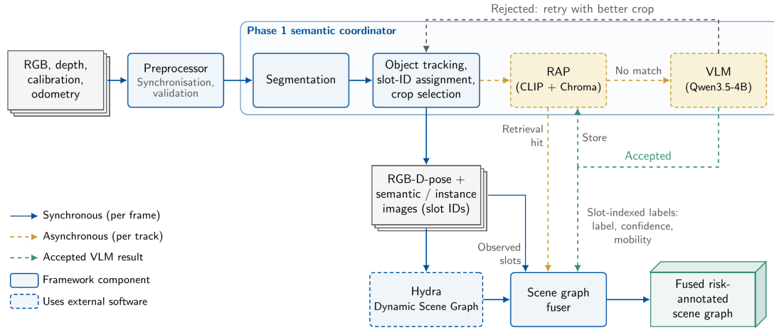
Figure 3.1.: Overview of the proposed framework, showing the synchronous per-frame path (solid) and the asynchronous per-track path (dashed).
