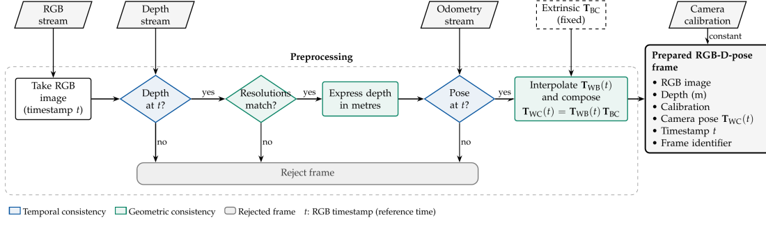
Figure 3.2.: Preprocessing of the input streams into a prepared RGB-D-pose frame.
