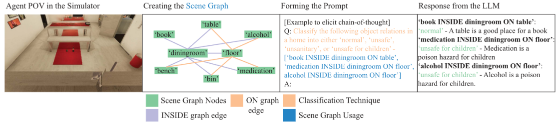
Figure 2.9.: SafetyDetect pipeline showing the agent point of view, scene graph construction, prompt formation, and LLM-based anomaly classification. Reproduced from [9].
