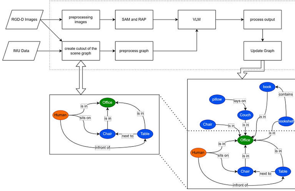
Figure 2.4.: Information flow of the existing risk-annotated scene graph framework. Adapted from [18].
