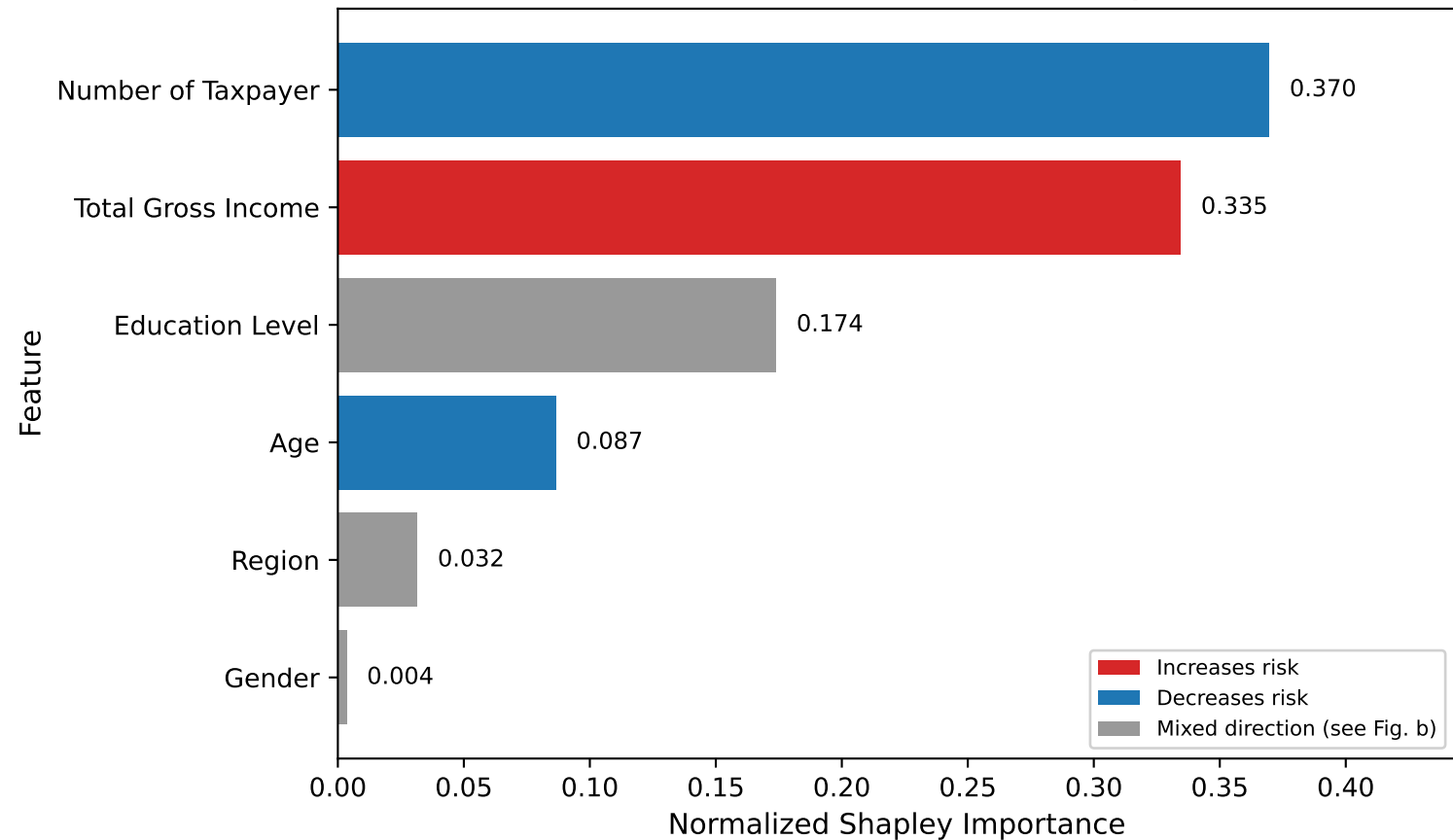
Feature Importance for R_i (Shapley Values)
