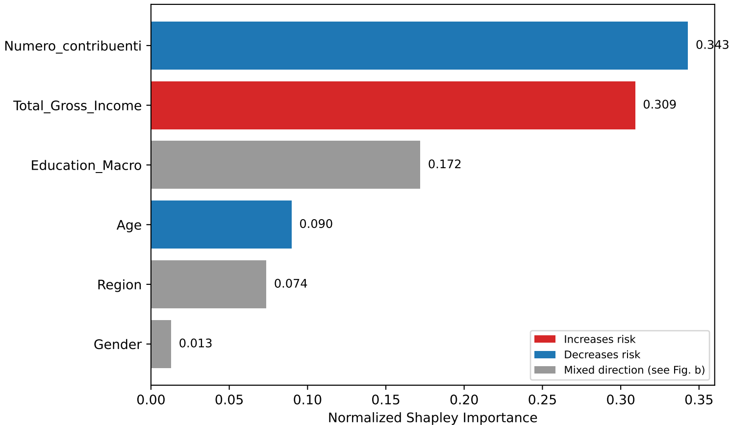
Feature Importance for R_i (Shapley Values) — XGBoost BIS
