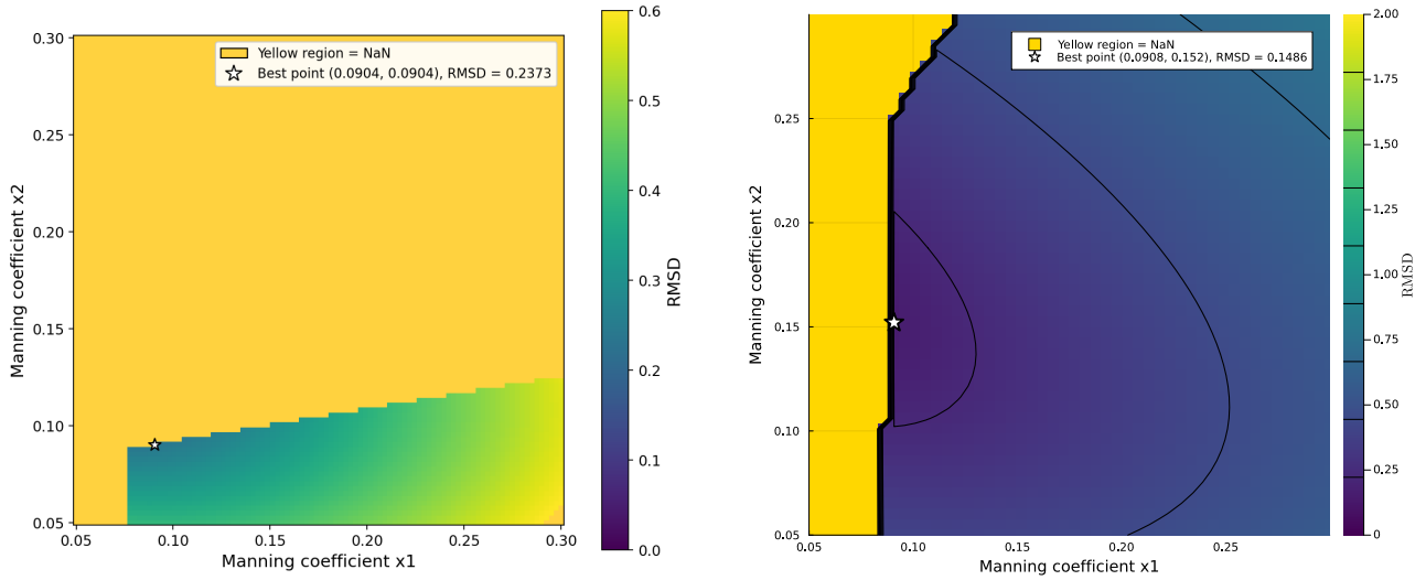
Figure 3: Comparison between the previous (left) and the current (right) PDE solver.
