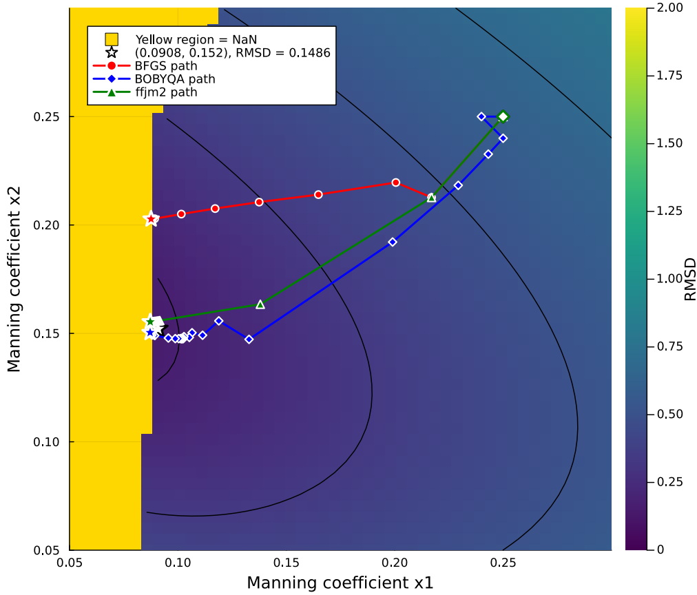
Figure 6: RMSD heatmap of the real-data experiment ( n_{\text{grid}} = 2 ) with the path of accepted iterates of each method overlaid: BFGS (red), BOBYQA (blue), and Algorithm ?? (green). The white diamond marks the shared starting point \xi^0 = (0.25, 0.25) ; the star marks each method’s final iterate.
