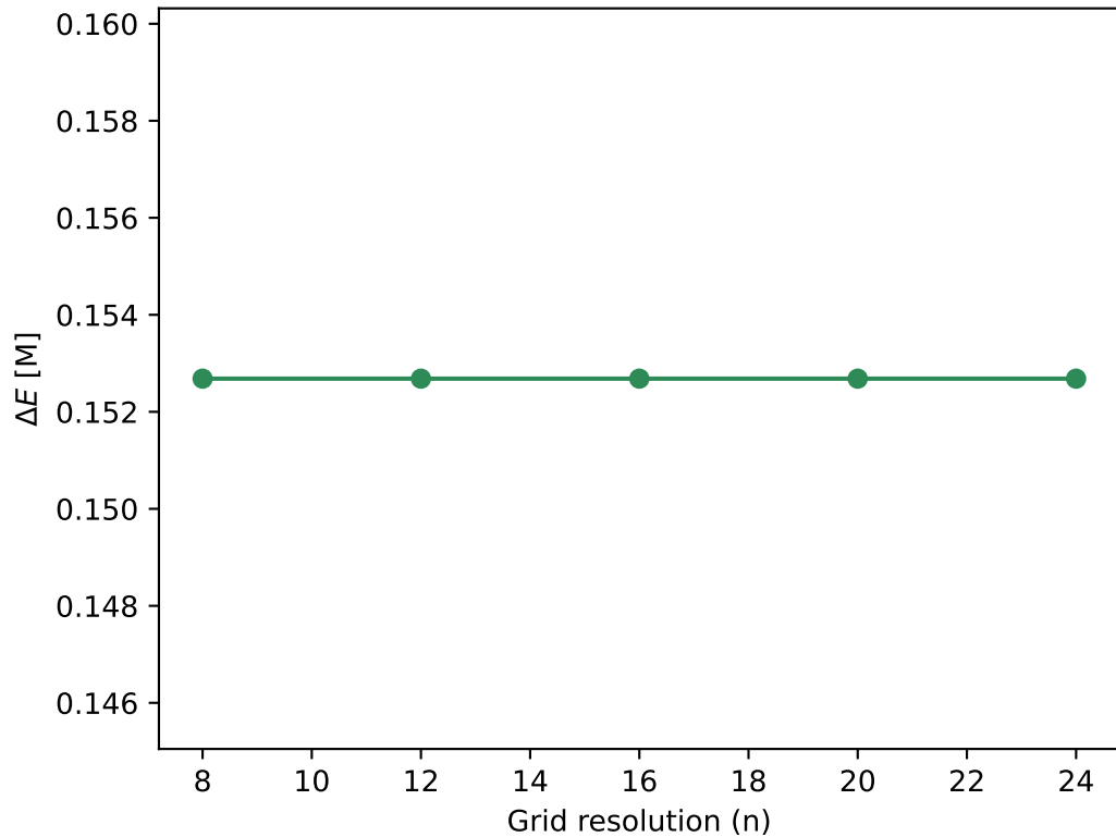
\Delta E convergence (a/M=0.9, static)
