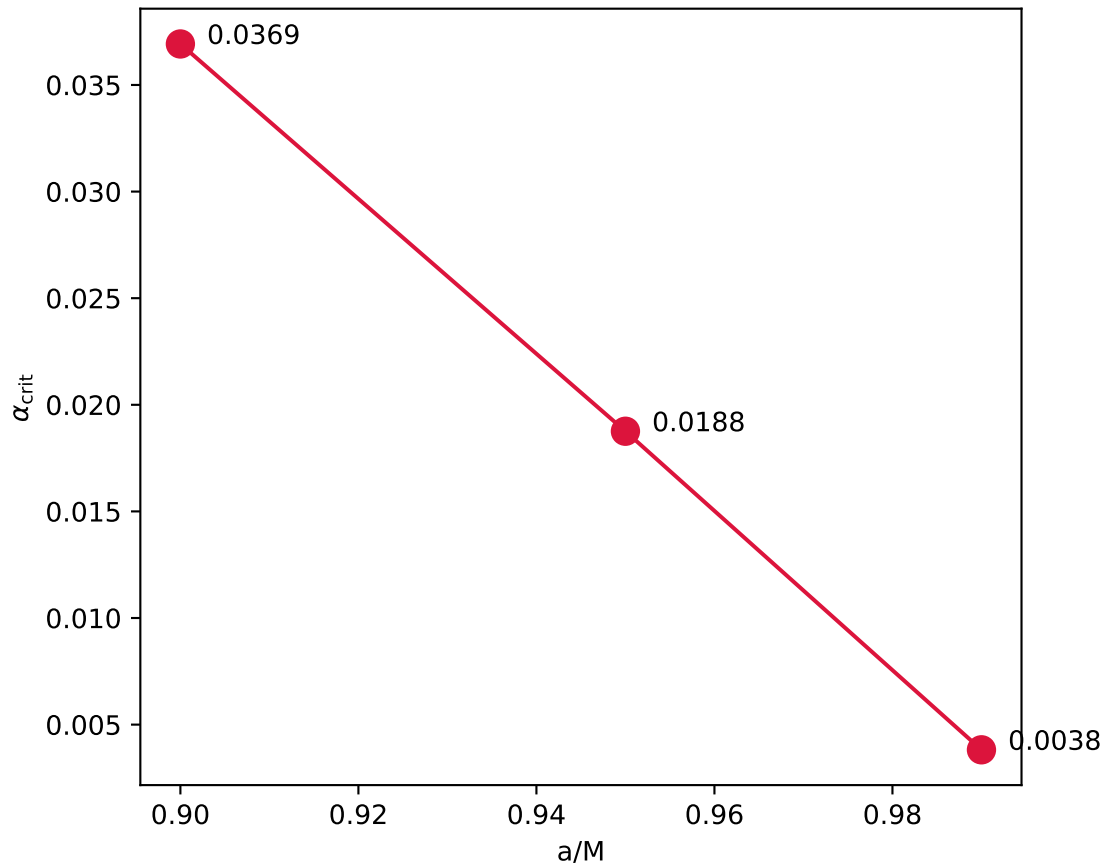
Phase boundary: \alpha_{\text{crit}} vs spin
