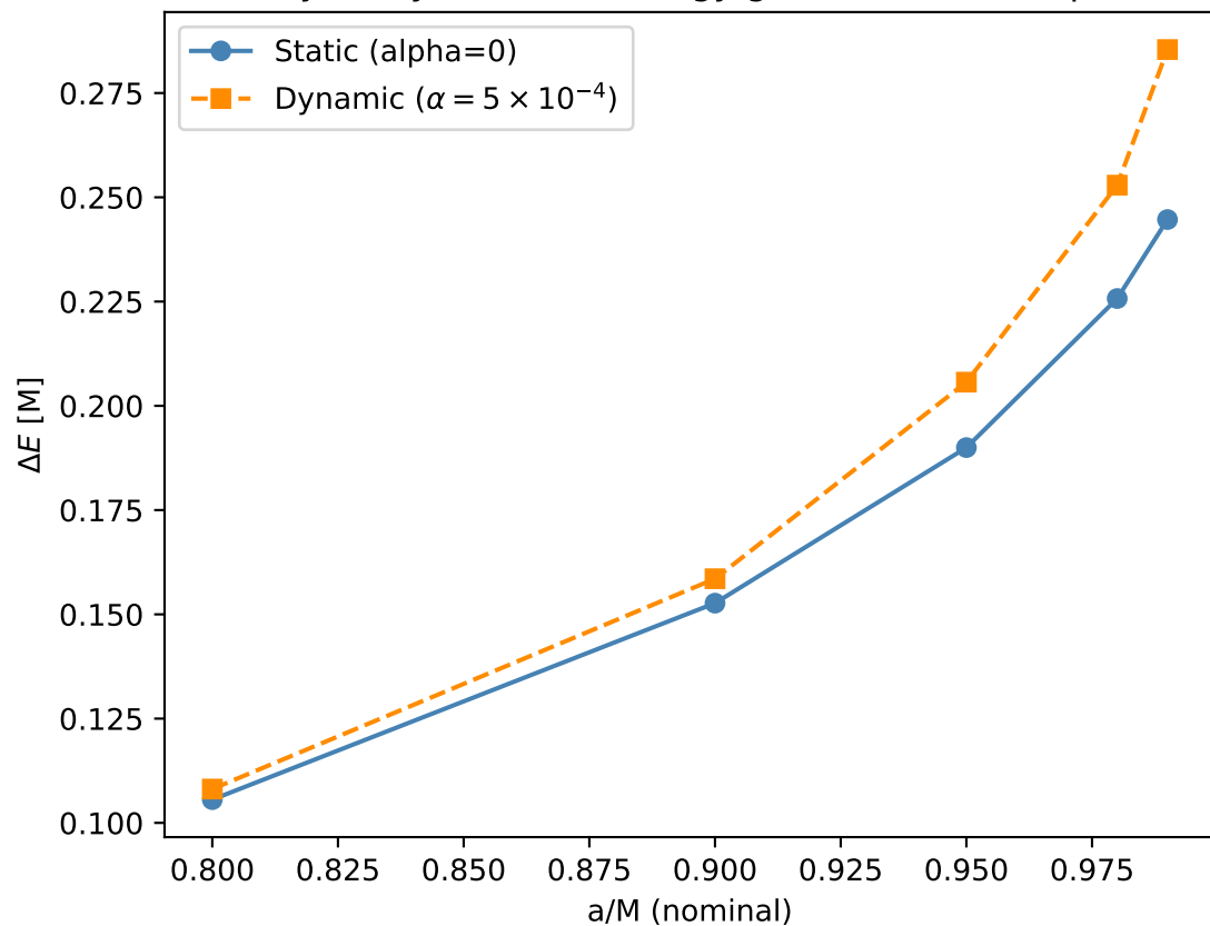
Physically bounded energy gain vs. nominal spin
