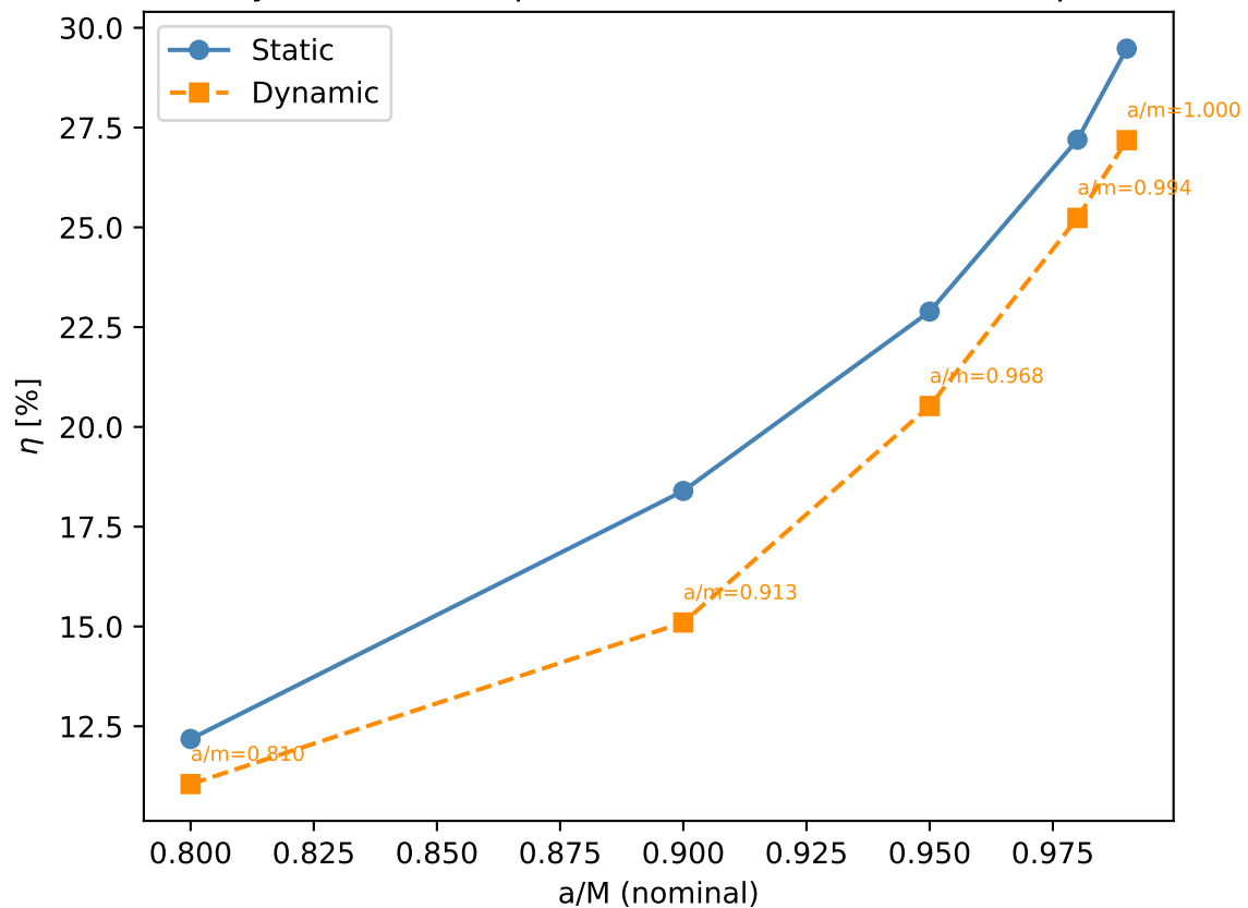
Efficiency vs. nominal spin (annotated: actual a/m at split time)
