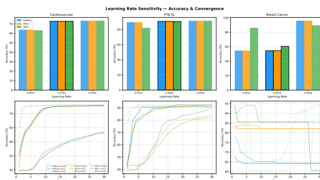
Fig. S-37. Learning rate sensitivity for top-3 algorithms (HPFL, Ditto, FedAvg). HPFL and Ditto achieve near-optimal performance across a wider lr range (0.005–0.01) compared to FedAvg.
