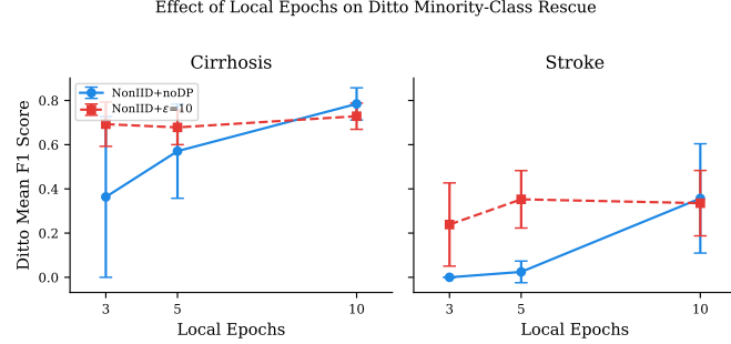
Fig. S-47. Effect of local epochs on Ditto minority-class F1. Cirrhosis shows monotonic improvement (0.36→0.57→0.78 for NonIID+noDP); Stroke improves dramatically at ep=10 (0.00→0.36), suggesting more local personalization steps help overcome extreme imbalance.
