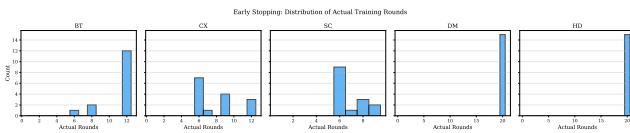
Fig. S-31. Early stopping analysis: actual rounds used vs. configured maximum. Most algorithms converge before the maximum round budget, demonstrating the effectiveness of patience-based early stopping.
