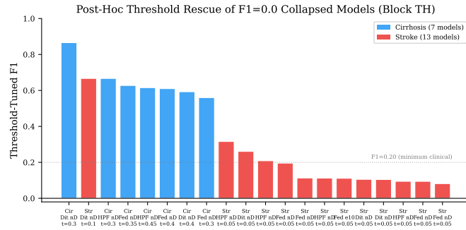
Fig. S-48. Post-hoc threshold rescue of F1=0.0 collapsed models. Cirrhosis models (blue) achieve clinically meaningful rescue (mean threshold-tuned F1=0.648); Stroke models (red) show marginal improvement (mean threshold-tuned F1=0.190), indicating insufficient minority-class signal.
