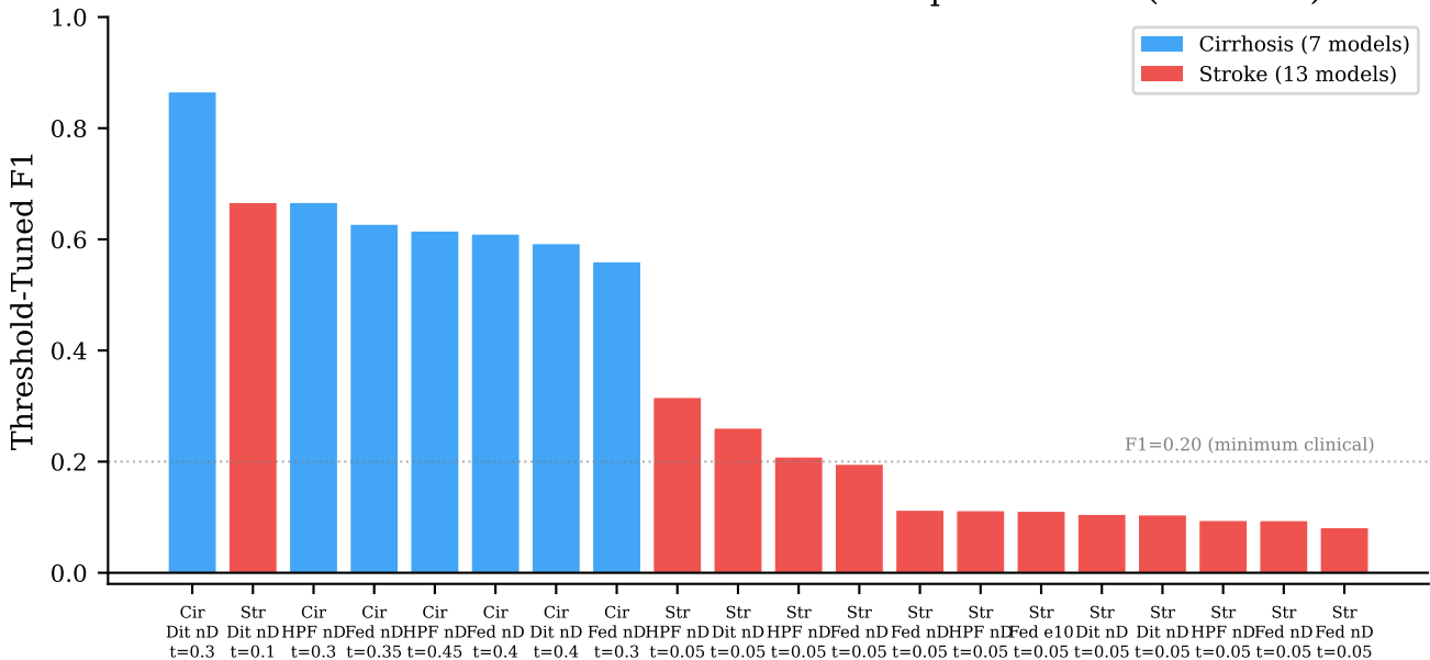
Post-Hoc Threshold Rescue of F1=0.0 Collapsed Models (Block TH)
