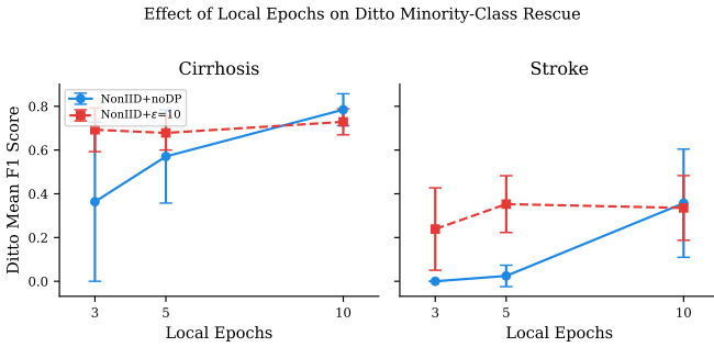
Fig. S-45. Effect of local epochs on Ditto minority-class F1. Cirrhosis shows monotonic improvement ( 0.36 \rightarrow 0.57 \rightarrow 0.78 for NonIID+noDP); Stroke improves dramatically at ep=10 ( 0.00 \rightarrow 0.36 ), suggesting more local personalization steps help overcome extreme imbalance.
