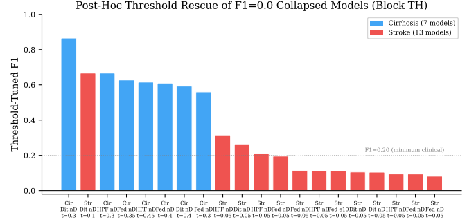
Fig. S-46. Post-hoc threshold rescue of F1=0.0 collapsed models. Cirrhosis models (blue) achieve clinically meaningful rescue (mean threshold-tuned F1=0.648); Stroke models (red) show marginal improvement (mean threshold-tuned F1=0.190), indicating insufficient minority-class signal.
