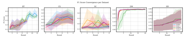
Fig. S-25. F1-score convergence over training rounds. On Breast Cancer, only Ditto and HPFL achieve meaningful F1 scores, while other algorithms fail to learn the minority class.
