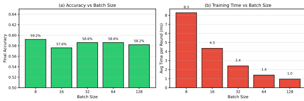
Fig. S-10. Batch size impact on convergence. Smaller batches (8–16) provide noisier gradients but faster initial progress. Batch size 32 balances gradient quality and computational efficiency.
